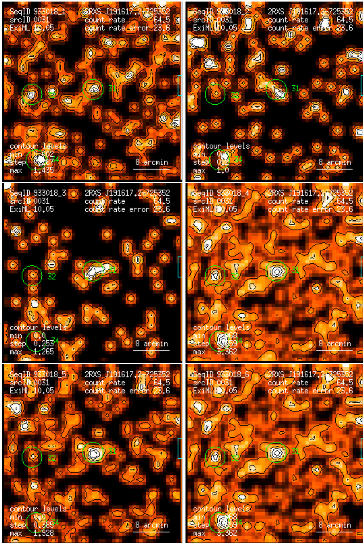
Figure 31: RASS 933018: detection 0031: band rate images, Gaussian filter: (1) PSPC channels 11 – 41, (2) 52 – 90, (3) 91 – 201, (4) 11 – 235, (5) 52 – 201, (6) 11 – 201. Broad band rates in counts/ks. Band rate contour levels in counts/ks/arcmin 2 .
