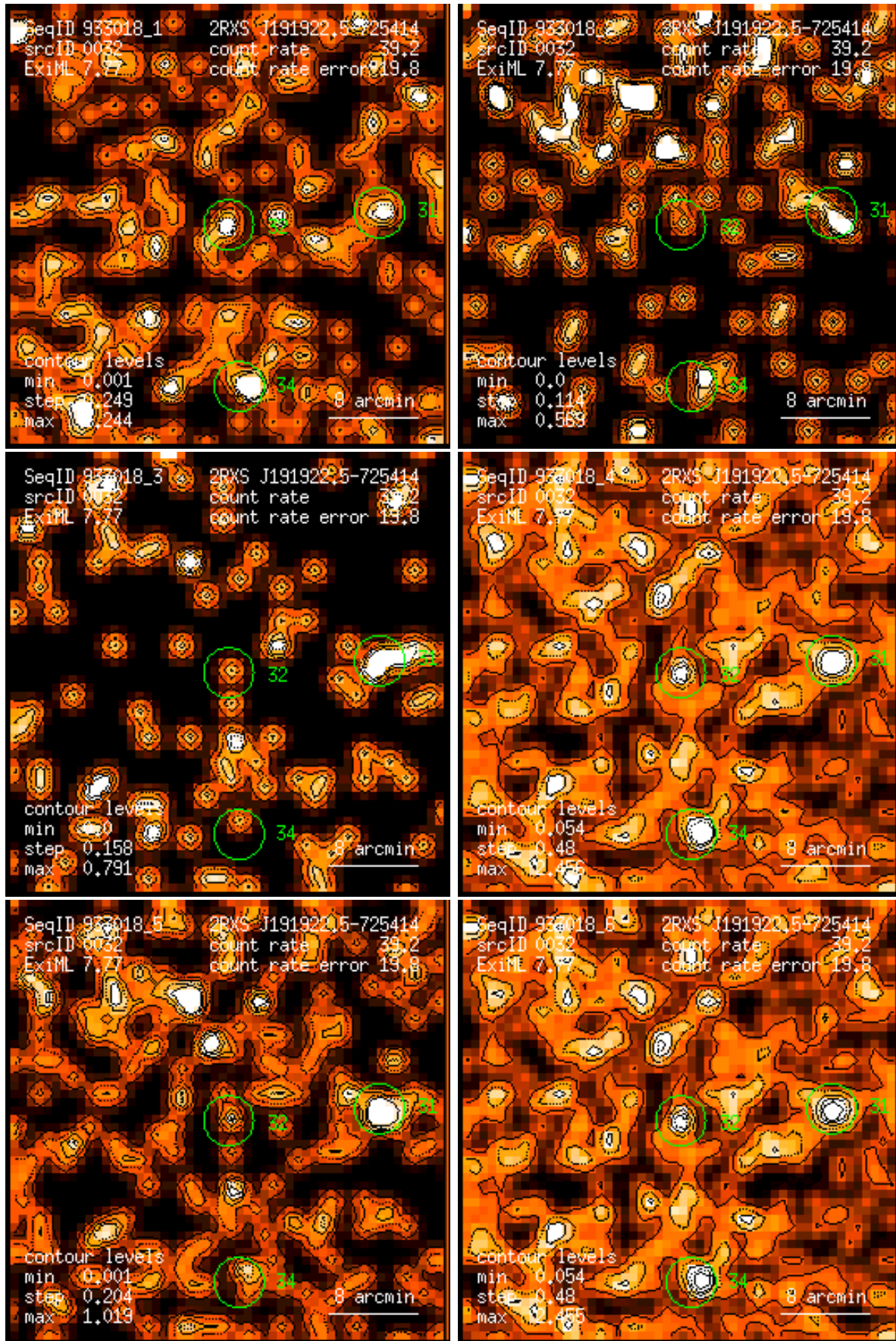
Figure 32: RASS 933018: detection 0032: band rate images, Gaussian filter: (1) PSPC channels 11 – 41, (2) 52 – 90, (3) 91 – 201, (4) 11 – 235, (5) 52 – 201, (6) 11 – 201. Broad band rates in counts/ks. Band rate contour levels in counts/ks/arcmin 2 .
