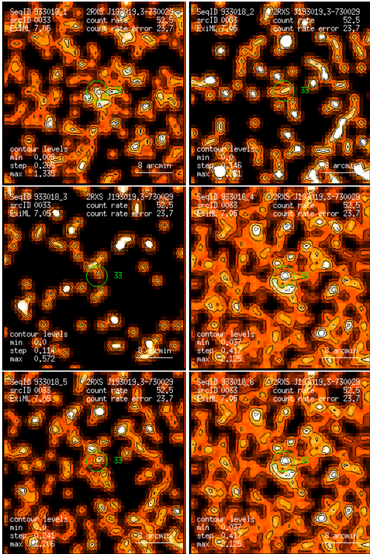
Figure 33: RASS 933018: detection 0033: band rate images, Gaussian filter: (1) PSPC channels 11 – 41, (2) 52 – 90, (3) 91 – 201, (4) 11 – 235, (5) 52 – 201, (6) 11 – 201. Broad band rates in counts/ks. Band rate contour levels in counts/ks/arcmin 2 .
