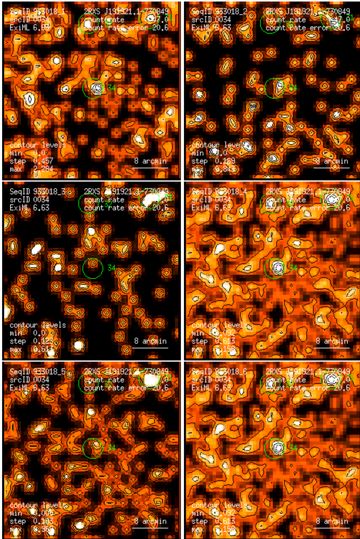
Figure 34: RASS 933018: detection 0034: band rate images, Gaussian filter: (1) PSPC channels 11 – 41, (2) 52 – 90, (3) 91 – 201, (4) 11 – 235, (5) 52 – 201, (6) 11 – 201. Broad band rates in counts/ks. Band rate contour levels in counts/ks/arcmin 2 .
