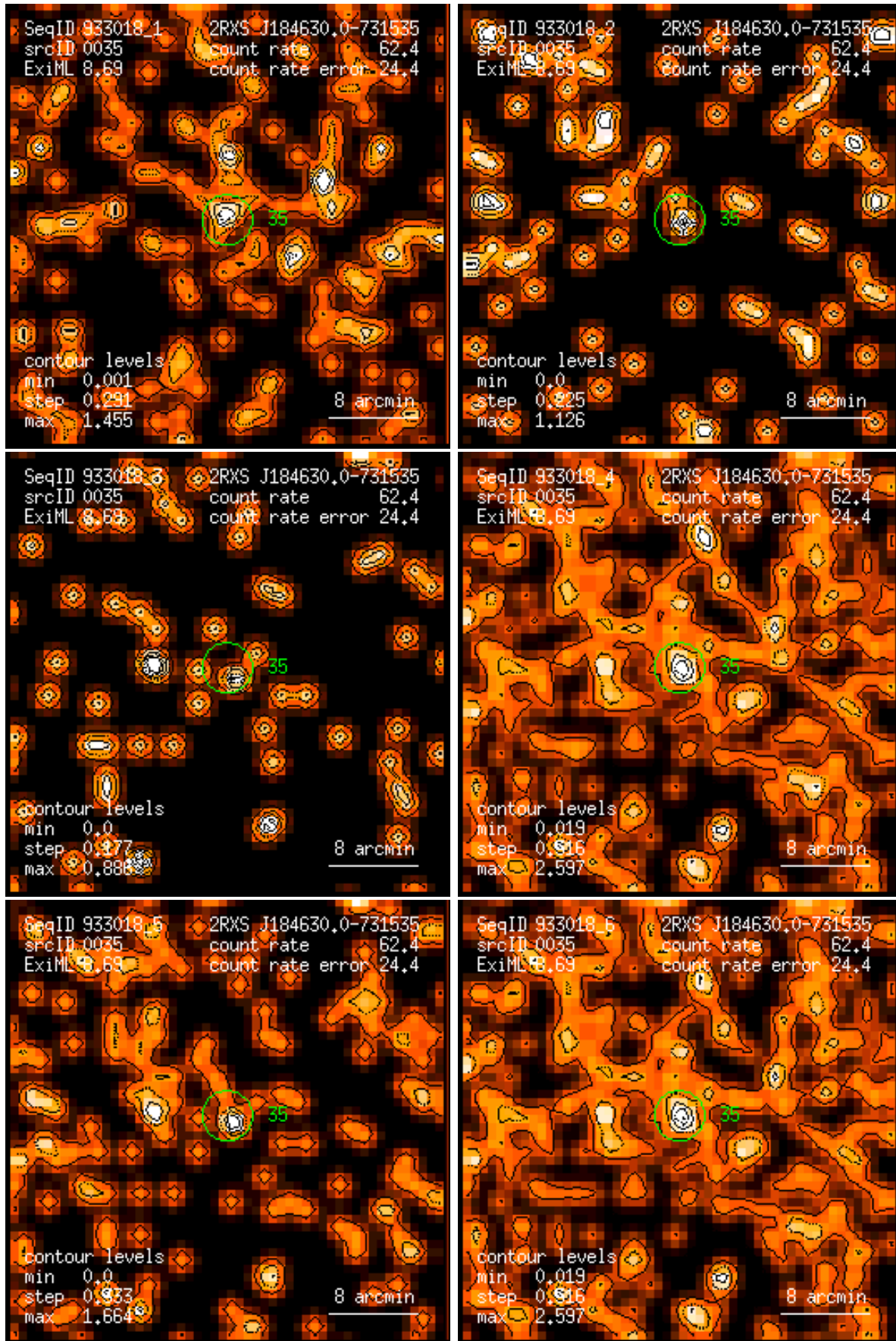
Figure 35: RASS 933018: detection 0035: band rate images, Gaussian filter: (1) PSPC channels 11 – 41, (2) 52 – 90, (3) 91 – 201, (4) 11 – 235, (5) 52 – 201, (6) 11 – 201. Broad band rates in counts/ks. Band rate contour levels in counts/ks/arcmin 2 .
