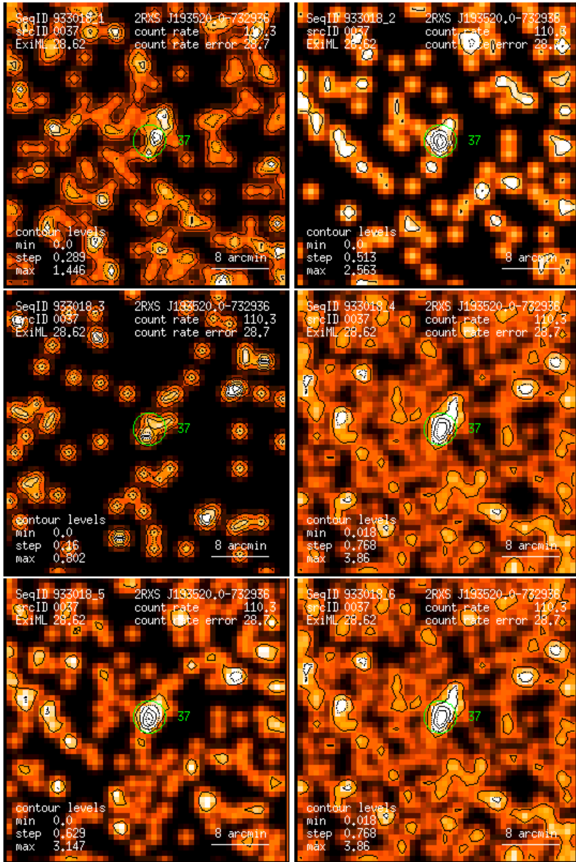
Figure 37: RASS 933018: detection 0037: band rate images, Gaussian filter: (1) PSPC channels 11 – 41, (2) 52 – 90, (3) 91 – 201, (4) 11 – 235, (5) 52 – 201, (6) 11 – 201. Broad band rates in counts/ks. Band rate contour levels in counts/ks/arcmin 2 .
