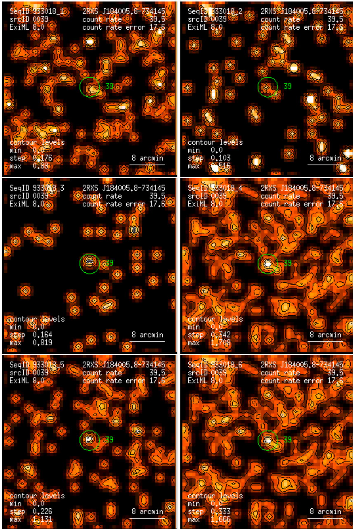
Figure 39: RASS 933018: detection 0039: band rate images, Gaussian filter: (1) PSPC channels 11 – 41, (2) 52 – 90, (3) 91 – 201, (4) 11 – 235, (5) 52 – 201, (6) 11 – 201. Broad band rates in counts/ks. Band rate contour levels in counts/ks/arcmin 2 .
