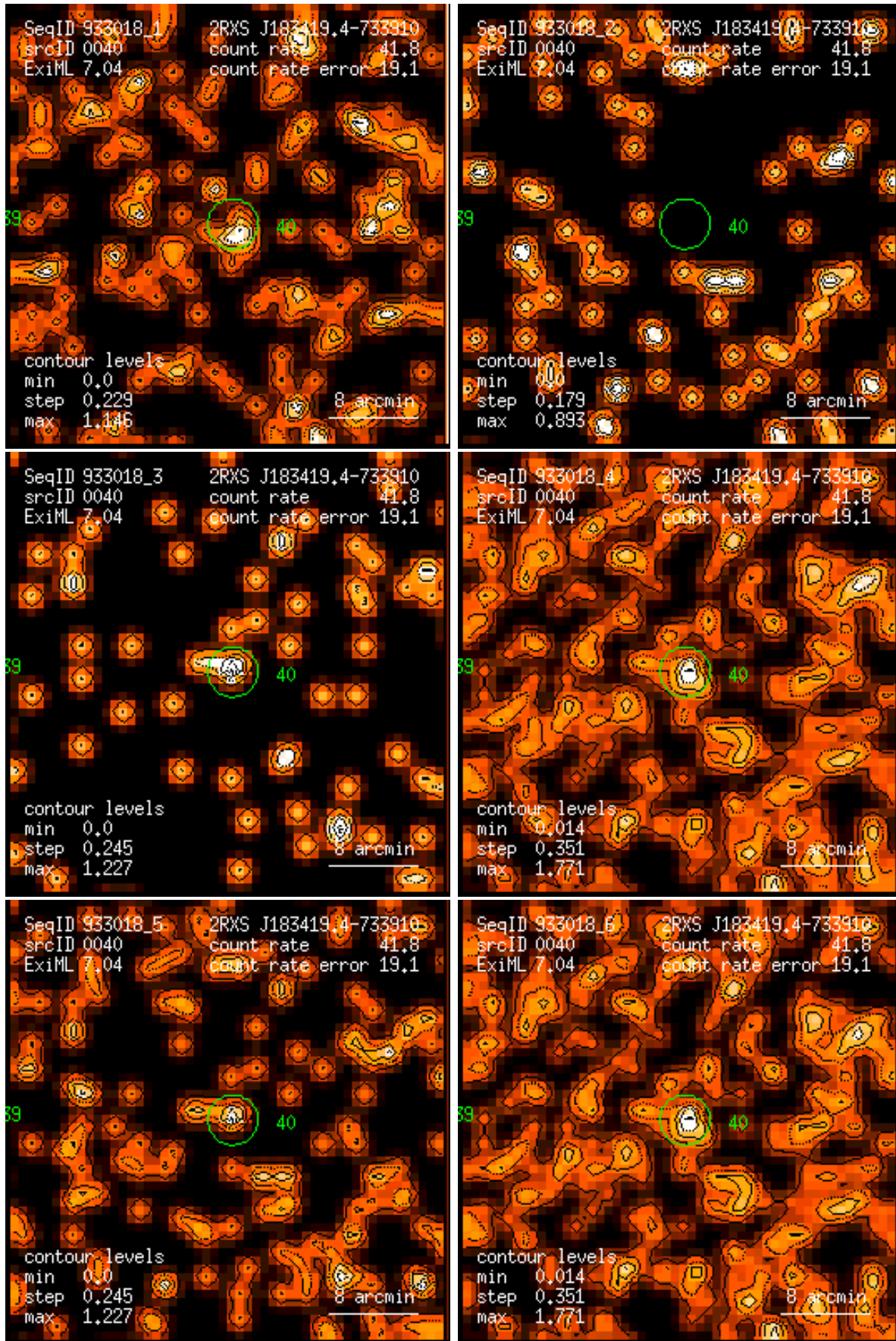
Figure 40: RASS 933018: detection 0040: band rate images, Gaussian filter: (1) PSPC channels 11 – 41, (2) 52 – 90, (3) 91 – 201, (4) 11 – 235, (5) 52 – 201, (6) 11 – 201. Broad band rates in counts/ks. Band rate contour levels in counts/ks/arcmin 2 .
