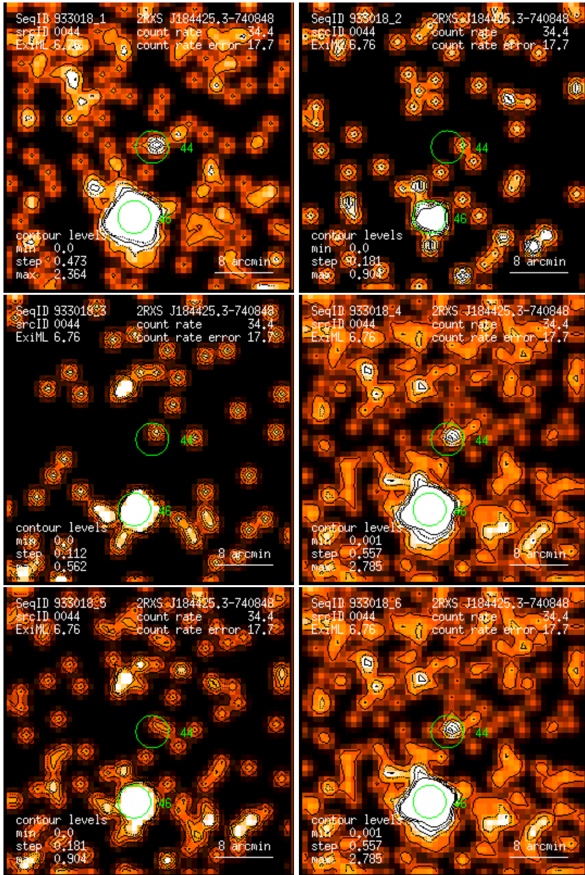
Figure 44: RASS 933018: detection 0044: band rate images, Gaussian filter: (1) PSPC channels 11 – 41, (2) 52 – 90, (3) 91 – 201, (4) 11 – 235, (5) 52 – 201, (6) 11 – 201. Broad band rates in counts/ks. Band rate contour levels in counts/ks/arcmin 2 .
