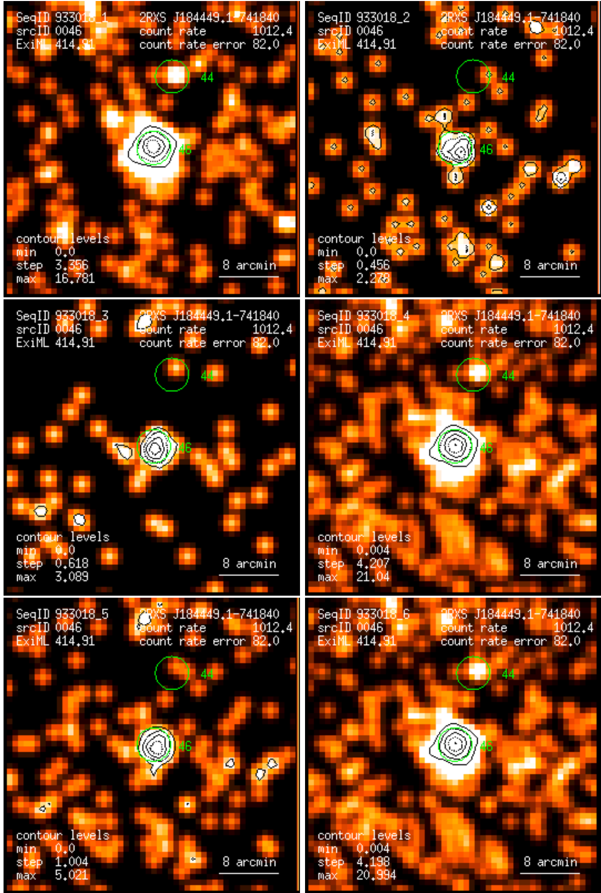
Figure 46: RASS 933018: detection 0046: band rate images, Gaussian filter: (1) PSPC channels 11 – 41, (2) 52 – 90, (3) 91 – 201, (4) 11 – 235, (5) 52 – 201, (6) 11 – 201. Broad band rates in counts/ks. Band rate contour levels in counts/ks/arcmin 2 .
