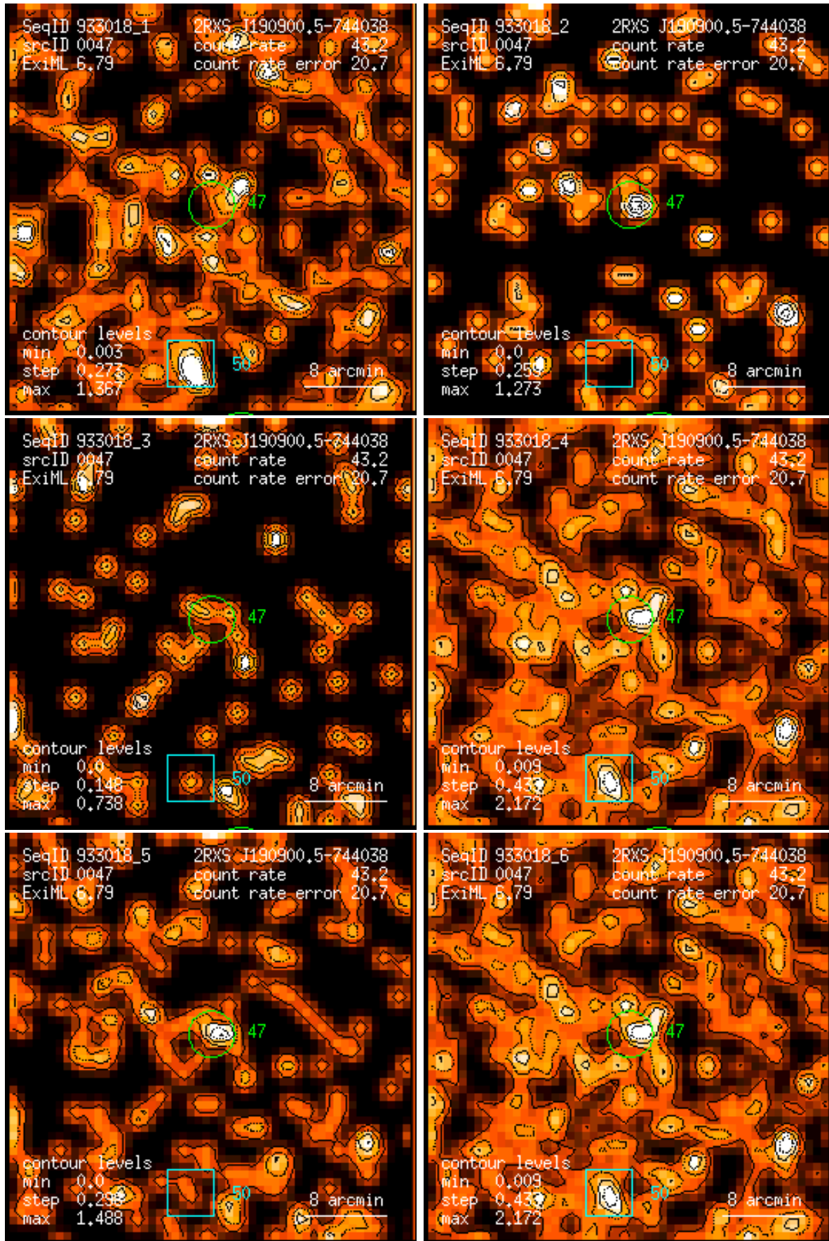
Figure 47: RASS 933018: detection 0047: band rate images, Gaussian filter: (1) PSPC channels 11 – 41, (2) 52 – 90, (3) 91 – 201, (4) 11 – 235, (5) 52 – 201, (6) 11 – 201. Broad band rates in counts/ks. Band rate contour levels in counts/ks/arcmin 2 .
