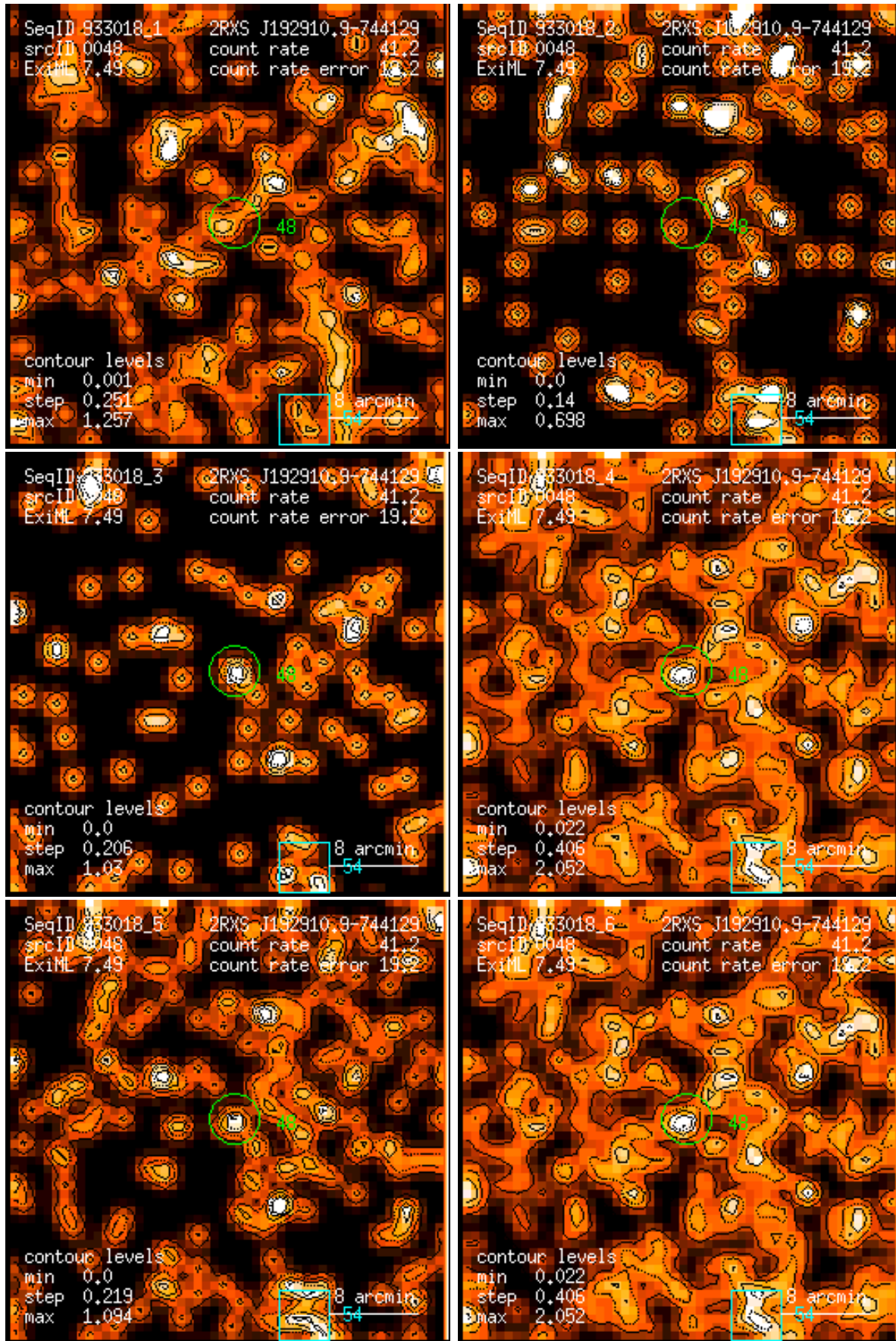
Figure 48: RASS 933018: detection 0048: band rate images, Gaussian filter: (1) PSPC channels 11 – 41, (2) 52 – 90, (3) 91 – 201, (4) 11 – 235, (5) 52 – 201, (6) 11 – 201. Broad band rates in counts/ks. Band rate contour levels in counts/ks/arcmin 2 .
