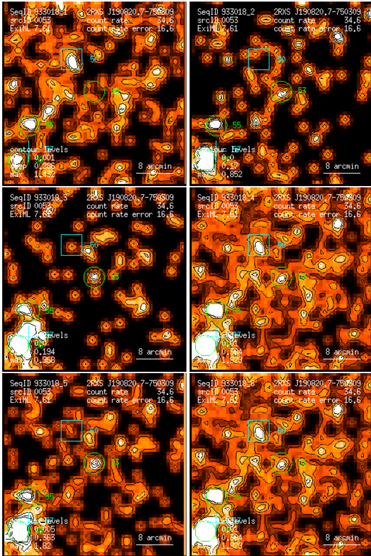
Figure 53: RASS 933018: detection 0053: band rate images, Gaussian filter: (1) PSPC channels 11 – 41, (2) 52 – 90, (3) 91 – 201, (4) 11 – 235, (5) 52 – 201, (6) 11 – 201. Broad band rates in counts/ks. Band rate contour levels in counts/ks/arcmin 2 .
