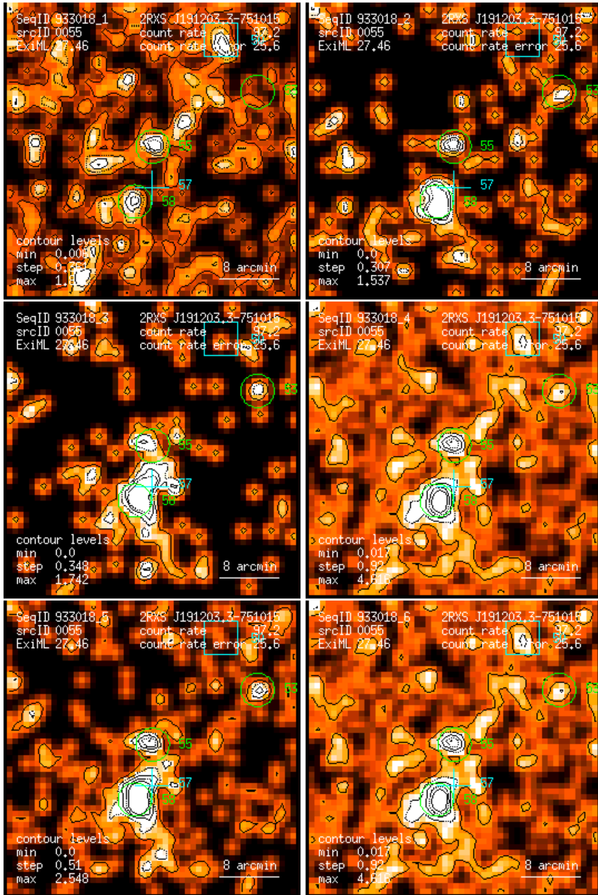
Figure 55: RASS 933018: detection 0055: band rate images, Gaussian filter: (1) PSPC channels 11 – 41, (2) 52 – 90, (3) 91 – 201, (4) 11 – 235, (5) 52 – 201, (6) 11 – 201. Broad band rates in counts/ks. Band rate contour levels in counts/ks/arcmin 2 .
