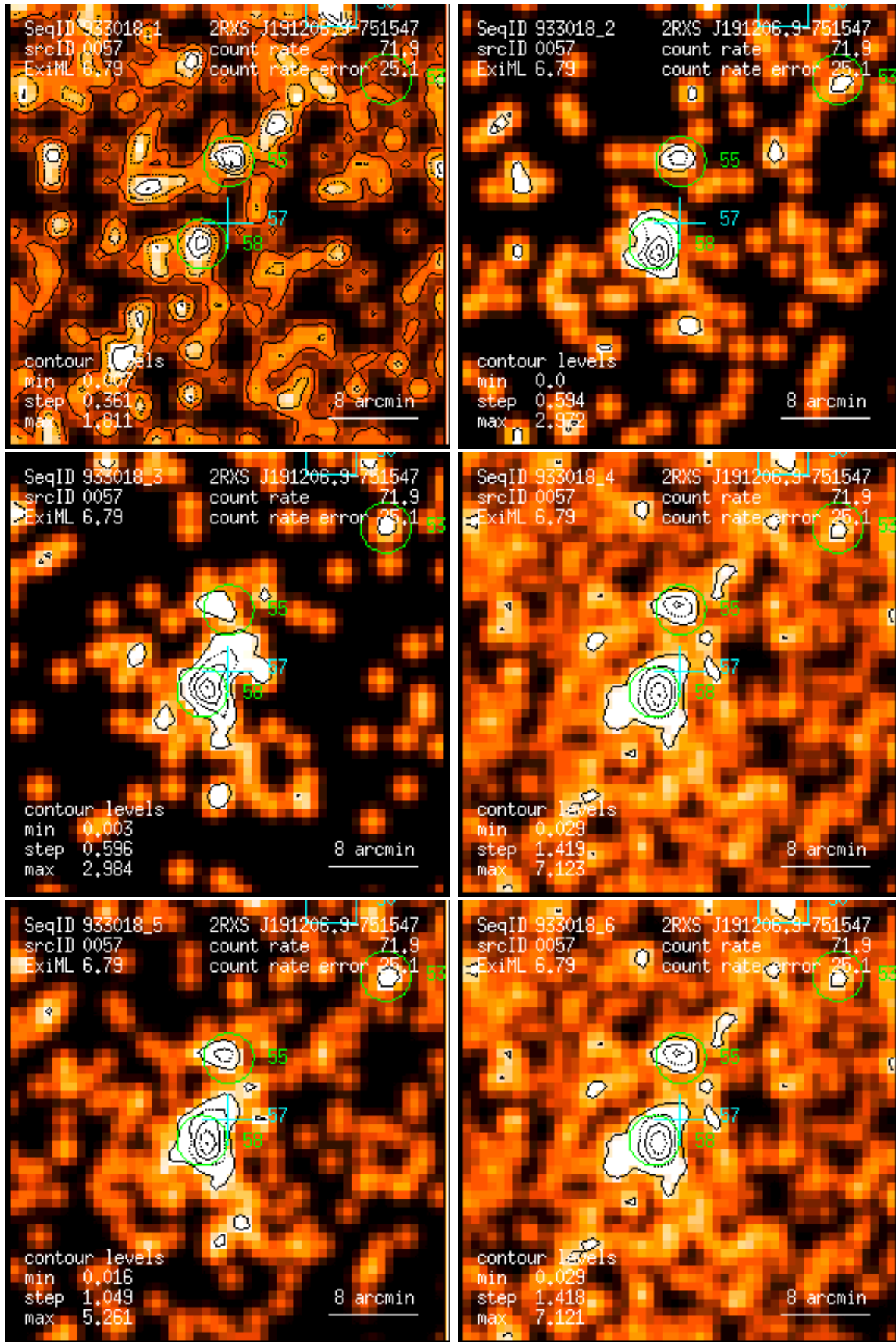
Figure 57: RASS 933018: detection 0057: band rate images, Gaussian filter: (1) PSPC channels 11 – 41, (2) 52 – 90, (3) 91 – 201, (4) 11 – 235, (5) 52 – 201, (6) 11 – 201. Broad band rates in counts/ks. Band rate contour levels in counts/ks/arcmin 2 .
