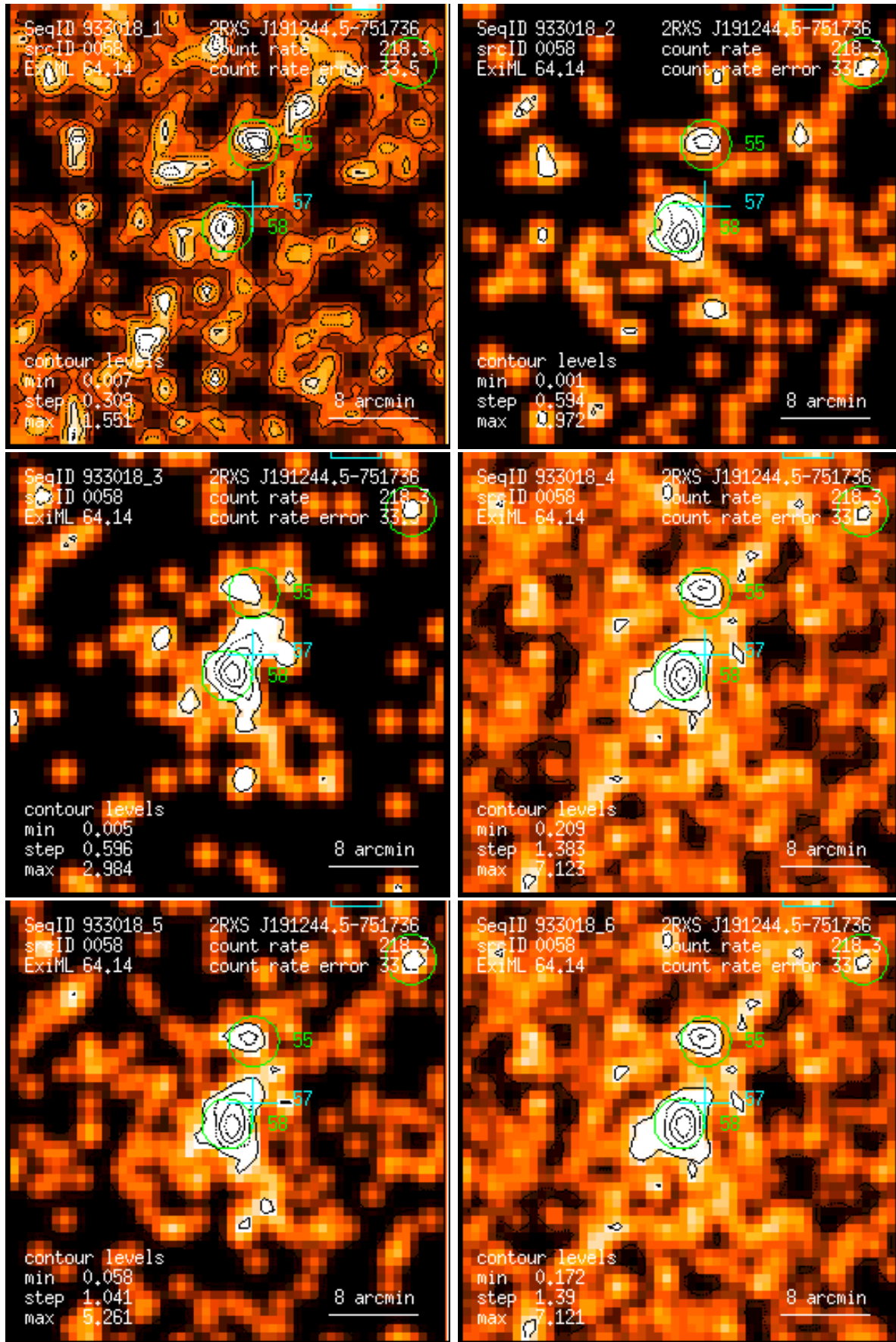
Figure 58: RASS 933018: detection 0058: band rate images, Gaussian filter: (1) PSPC channels 11 – 41, (2) 52 – 90, (3) 91 – 201, (4) 11 – 235, (5) 52 – 201, (6) 11 – 201. Broad band rates in counts/ks. Band rate contour levels in counts/ks/arcmin 2 .
