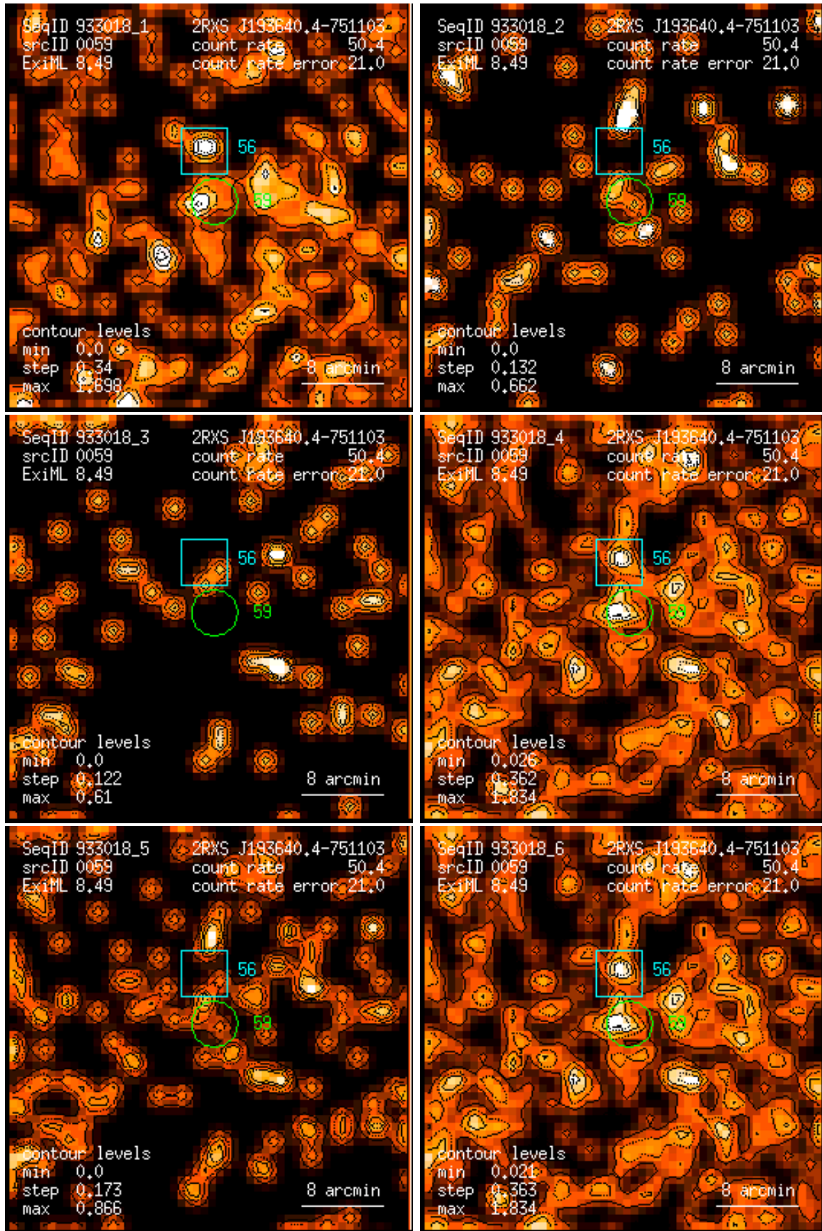
Figure 59: RASS 933018: detection 0059: band rate images, Gaussian filter: (1) PSPC channels 11 – 41, (2) 52 – 90, (3) 91 – 201, (4) 11 – 235, (5) 52 – 201, (6) 11 – 201. Broad band rates in counts/ks. Band rate contour levels in counts/ks/arcmin 2 .
