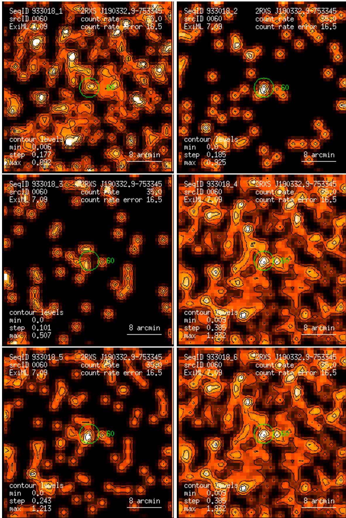
Figure 60: RASS 933018: detection 0060: band rate images, Gaussian filter: (1) PSPC channels 11 – 41, (2) 52 – 90, (3) 91 – 201, (4) 11 – 235, (5) 52 – 201, (6) 11 – 201. Broad band rates in counts/ks. Band rate contour levels in counts/ks/arcmin 2 .
