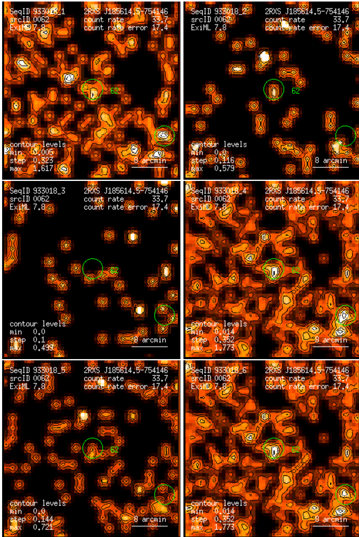
Figure 62: RASS 933018: detection 0062: band rate images, Gaussian filter: (1) PSPC channels 11 – 41, (2) 52 – 90, (3) 91 – 201, (4) 11 – 235, (5) 52 – 201, (6) 11 – 201. Broad band rates in counts/ks. Band rate contour levels in counts/ks/arcmin 2 .
