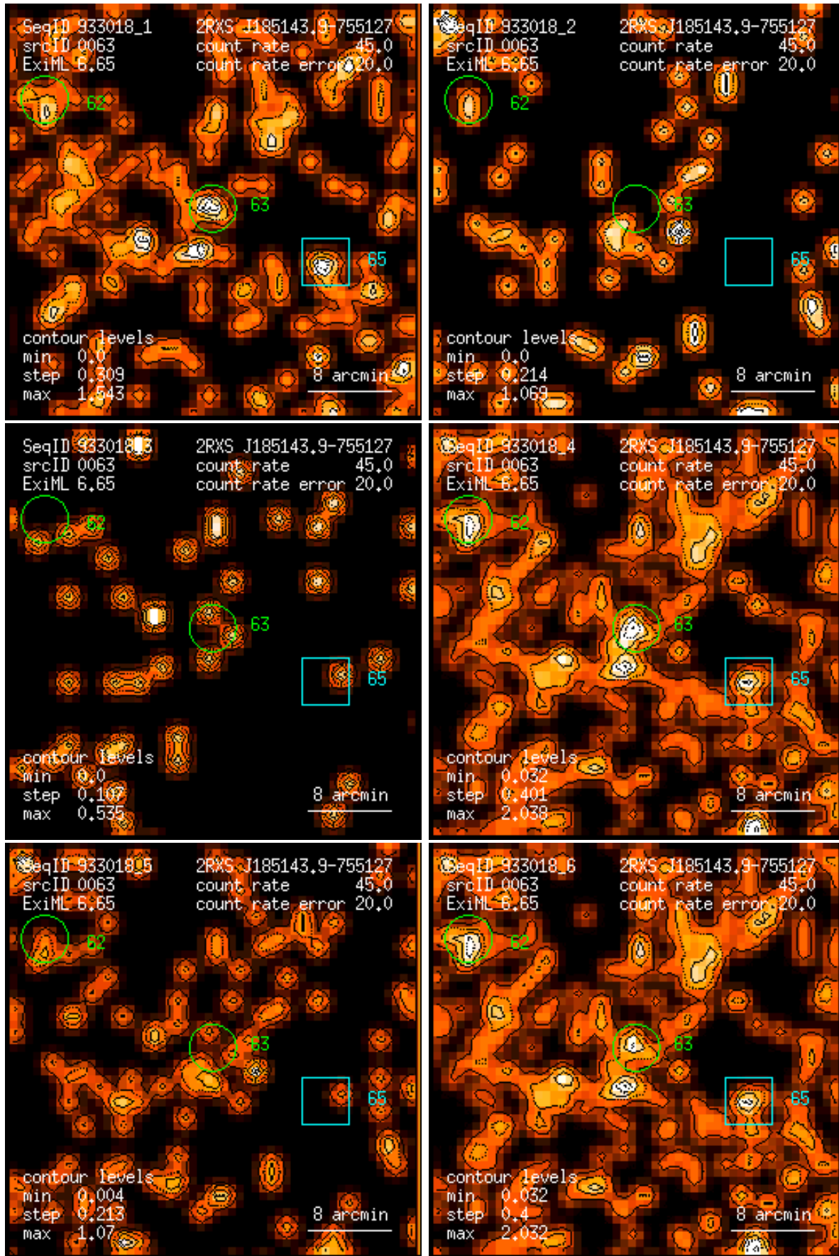
Figure 63: RASS 933018: detection 0063: band rate images, Gaussian filter: (1) PSPC channels 11 – 41, (2) 52 – 90, (3) 91 – 201, (4) 11 – 235, (5) 52 – 201, (6) 11 – 201. Broad band rates in counts/ks. Band rate contour levels in counts/ks/arcmin 2 .
