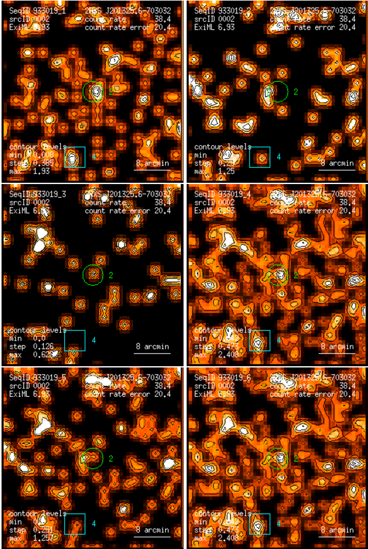
Figure 2: RASS 933019: detection 0002: band rate images, Gaussian filter: (1) PSPC channels 11 – 41, (2) 52 – 90, (3) 91 – 201, (4) 11 – 235, (5) 52 – 201, (6) 11 – 201. Broad band rates in counts/ks. Band rate contour levels in counts/ks/arcmin 2 .
