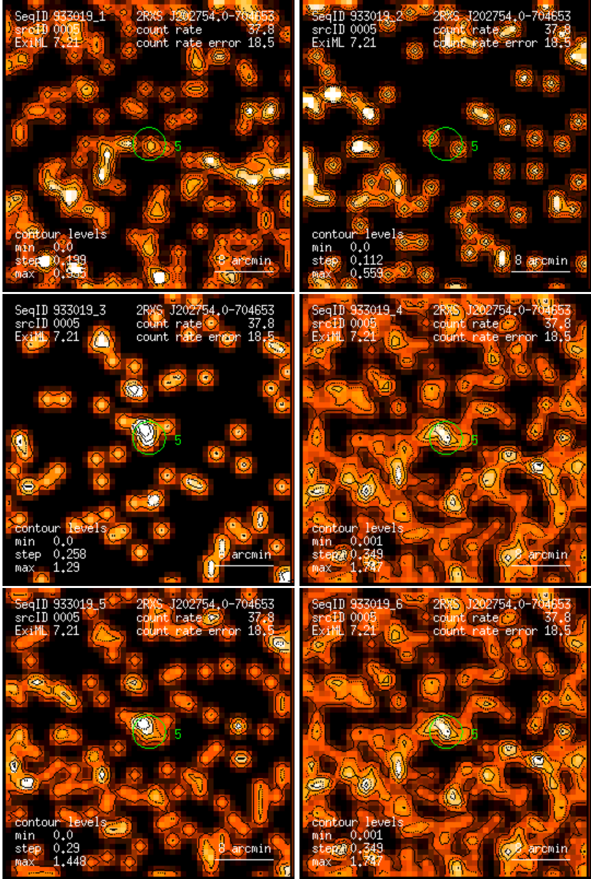
Figure 5: RASS 933019: detection 0005: band rate images, Gaussian filter: (1) PSPC channels 11 – 41, (2) 52 – 90, (3) 91 – 201, (4) 11 – 235, (5) 52 – 201, (6) 11 – 201. Broad band rates in counts/ks. Band rate contour levels in counts/ks/arcmin 2 .
