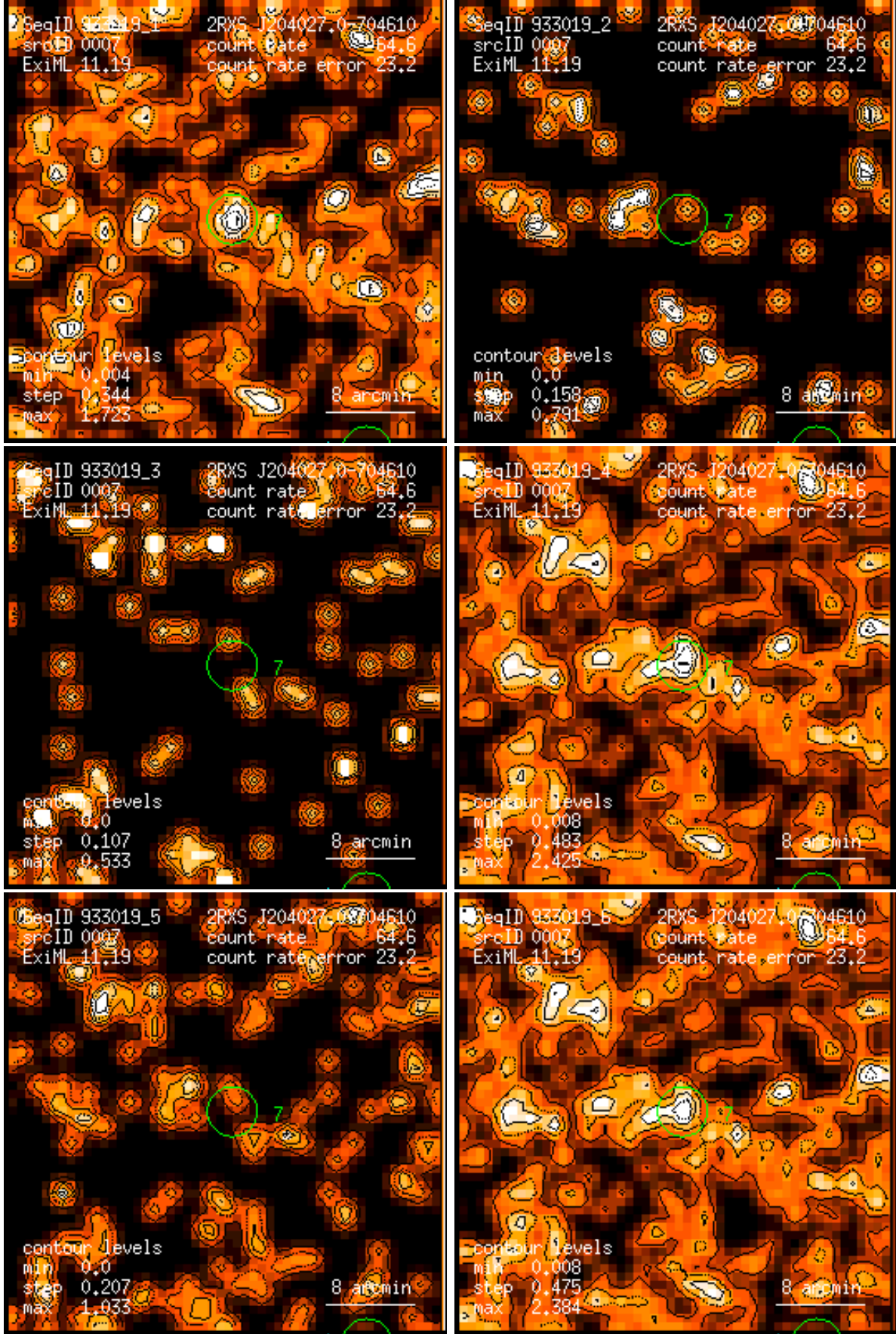
Figure 7: RASS 933019: detection 0007: band rate images, Gaussian filter: (1) PSPC channels 11 – 41, (2) 52 – 90, (3) 91 – 201, (4) 11 – 235, (5) 52 – 201, (6) 11 – 201. Broad band rates in counts/ks. Band rate contour levels in counts/ks/arcmin 2 .
