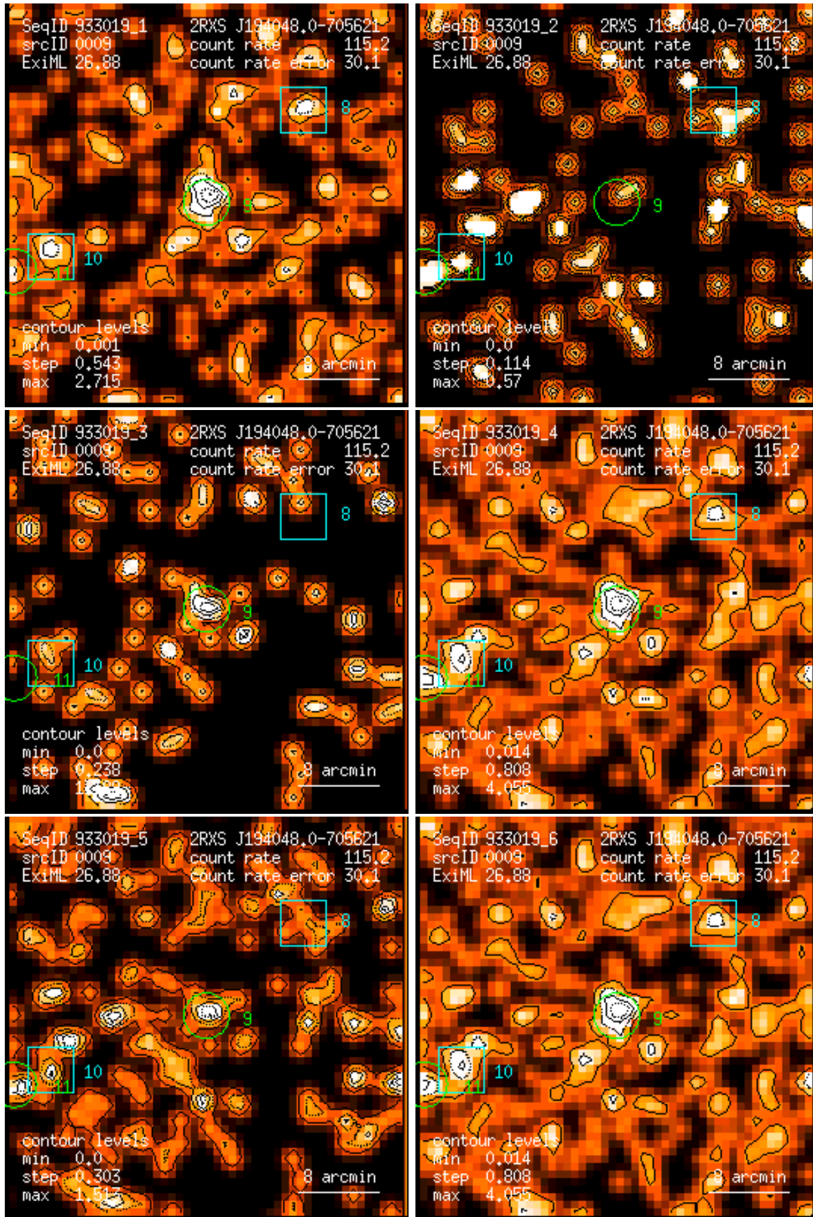
Figure 9: RASS 933019: detection 0009: band rate images, Gaussian filter: (1) PSPC channels 11 – 41, (2) 52 – 90, (3) 91 – 201, (4) 11 – 235, (5) 52 – 201, (6) 11 – 201. Broad band rates in counts/ks. Band rate contour levels in counts/ks/arcmin 2 .
