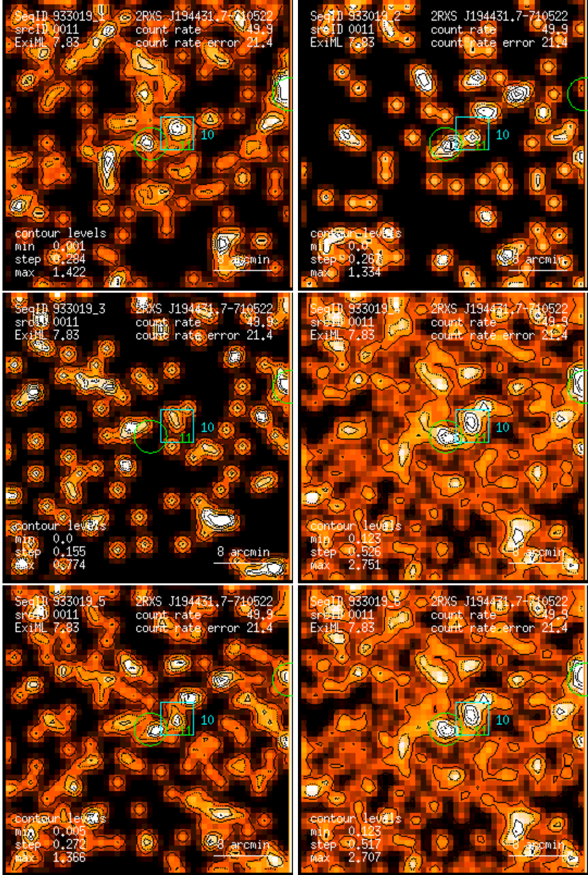
Figure 11: RASS 933019: detection 0011: band rate images, Gaussian filter: (1) PSPC channels 11 – 41, (2) 52 – 90, (3) 91 – 201, (4) 11 – 235, (5) 52 – 201, (6) 11 – 201. Broad band rates in counts/ks. Band rate contour levels in counts/ks/arcmin 2 .
