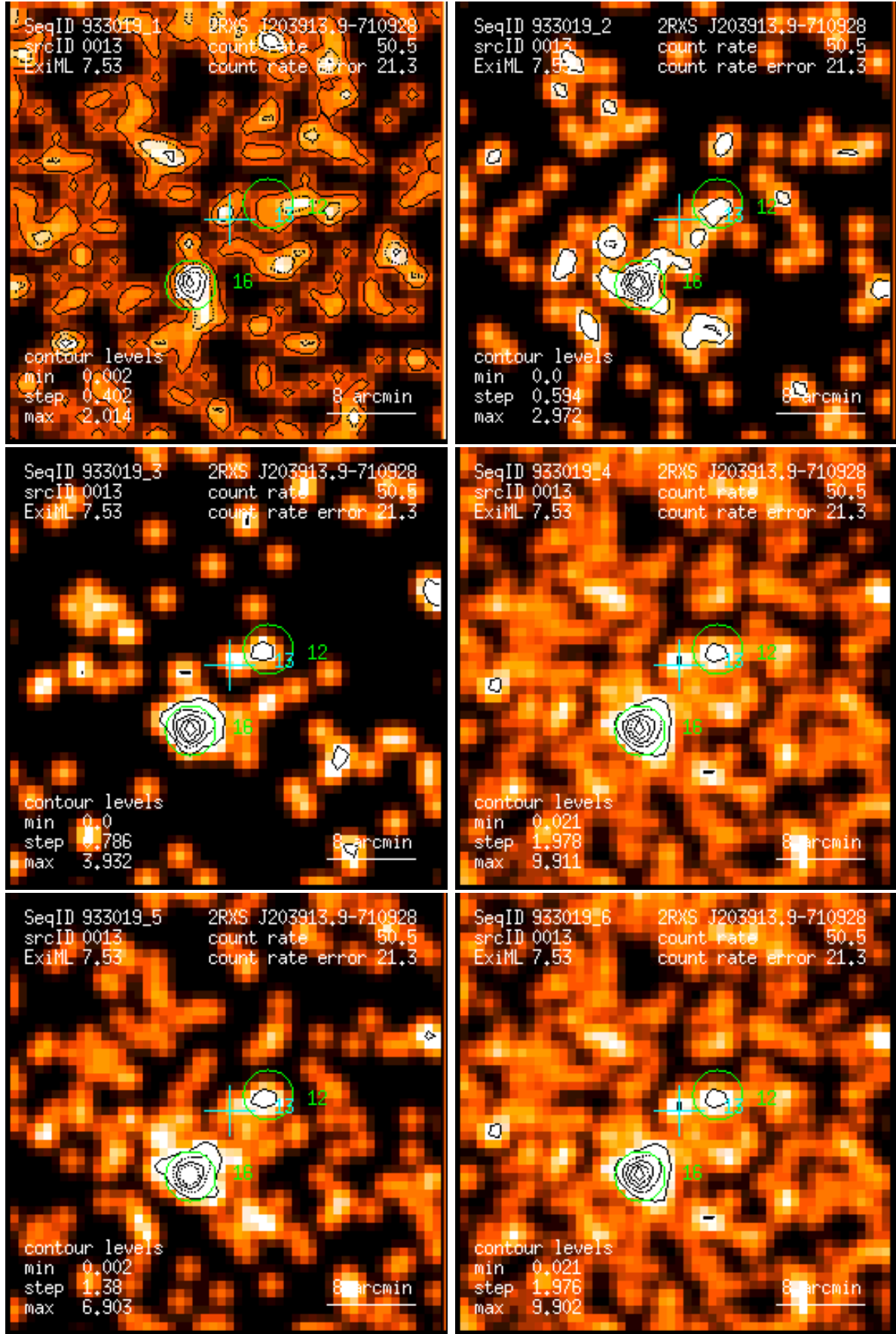
Figure 13: RASS 933019: detection 0013: band rate images, Gaussian filter: (1) PSPC channels 11 – 41, (2) 52 – 90, (3) 91 – 201, (4) 11 – 235, (5) 52 – 201, (6) 11 – 201. Broad band rates in counts/ks. Band rate contour levels in counts/ks/arcmin 2 .
