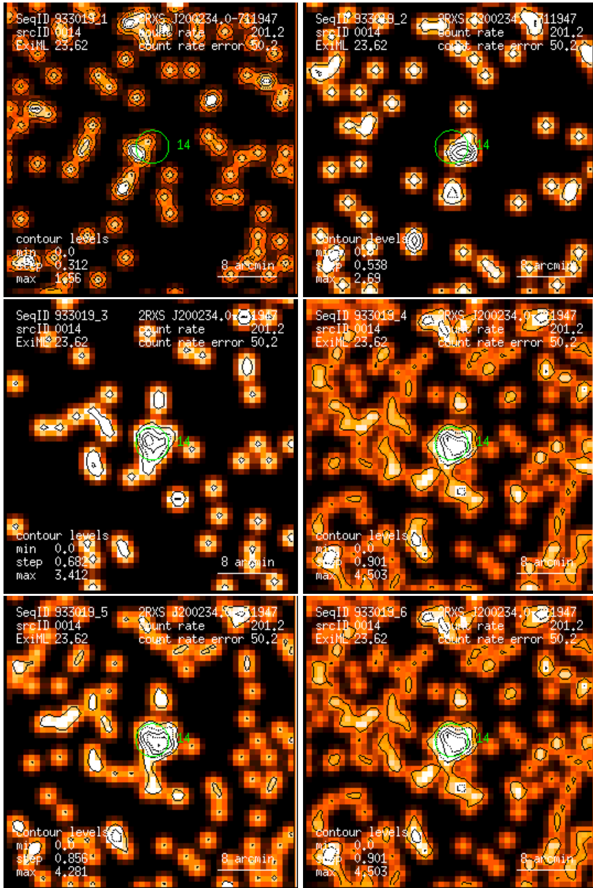
Figure 14: RASS 933019: detection 0014: band rate images, Gaussian filter: (1) PSPC channels 11 – 41, (2) 52 – 90, (3) 91 – 201, (4) 11 – 235, (5) 52 – 201, (6) 11 – 201. Broad band rates in counts/ks. Band rate contour levels in counts/ks/arcmin 2 .
