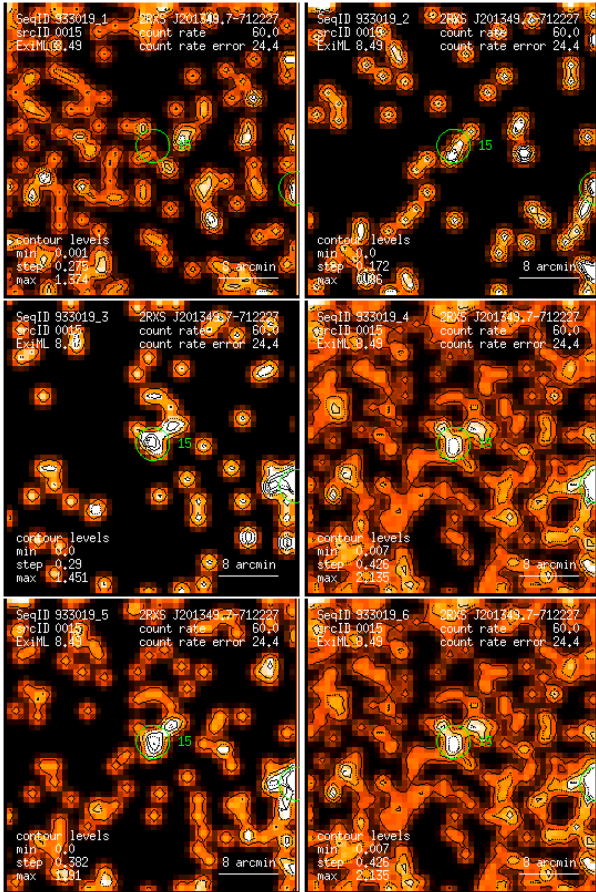
Figure 15: RASS 933019: detection 0015: band rate images, Gaussian filter: (1) PSPC channels 11 – 41, (2) 52 – 90, (3) 91 – 201, (4) 11 – 235, (5) 52 – 201, (6) 11 – 201. Broad band rates in counts/ks. Band rate contour levels in counts/ks/arcmin 2 .
