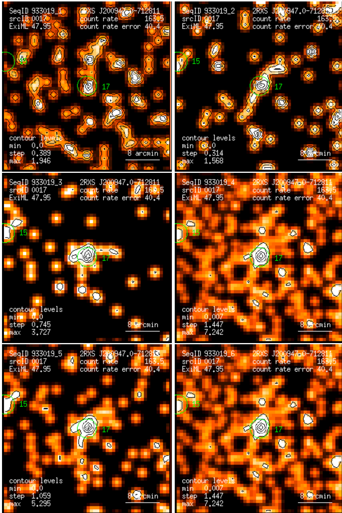
Figure 17: RASS 933019: detection 0017: band rate images, Gaussian filter: (1) PSPC channels 11 – 41, (2) 52 – 90, (3) 91 – 201, (4) 11 – 235, (5) 52 – 201, (6) 11 – 201. Broad band rates in counts/ks. Band rate contour levels in counts/ks/arcmin 2 .
