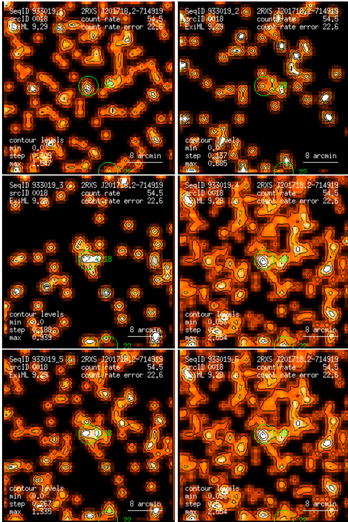
Figure 18: RASS 933019: detection 0018: band rate images, Gaussian filter: (1) PSPC channels 11 – 41, (2) 52 – 90, (3) 91 – 201, (4) 11 – 235, (5) 52 – 201, (6) 11 – 201. Broad band rates in counts/ks. Band rate contour levels in counts/ks/arcmin 2 .
