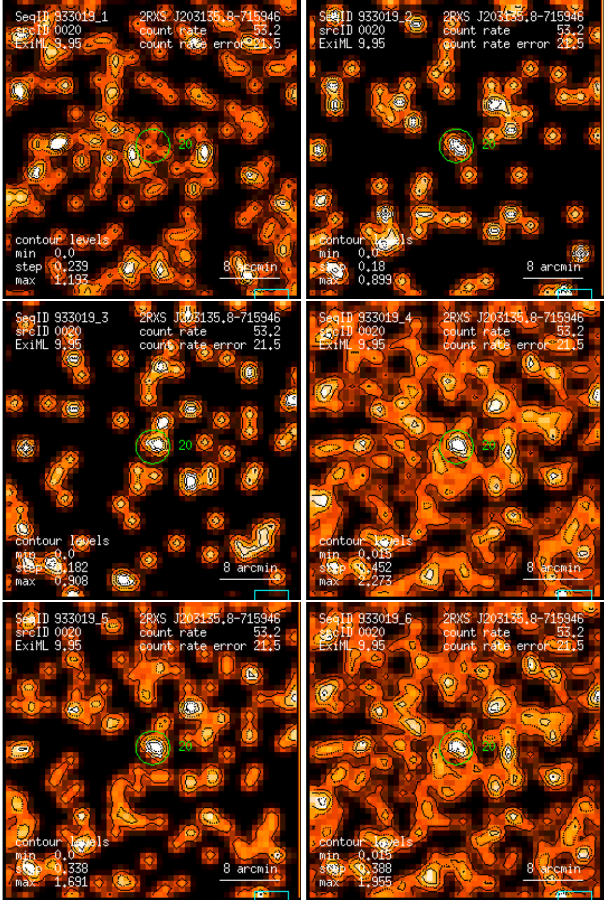
Figure 20: RASS 933019: detection 0020: band rate images, Gaussian filter: (1) PSPC channels 11 – 41, (2) 52 – 90, (3) 91 – 201, (4) 11 – 235, (5) 52 – 201, (6) 11 – 201. Broad band rates in counts/ks. Band rate contour levels in counts/ks/arcmin 2 .
