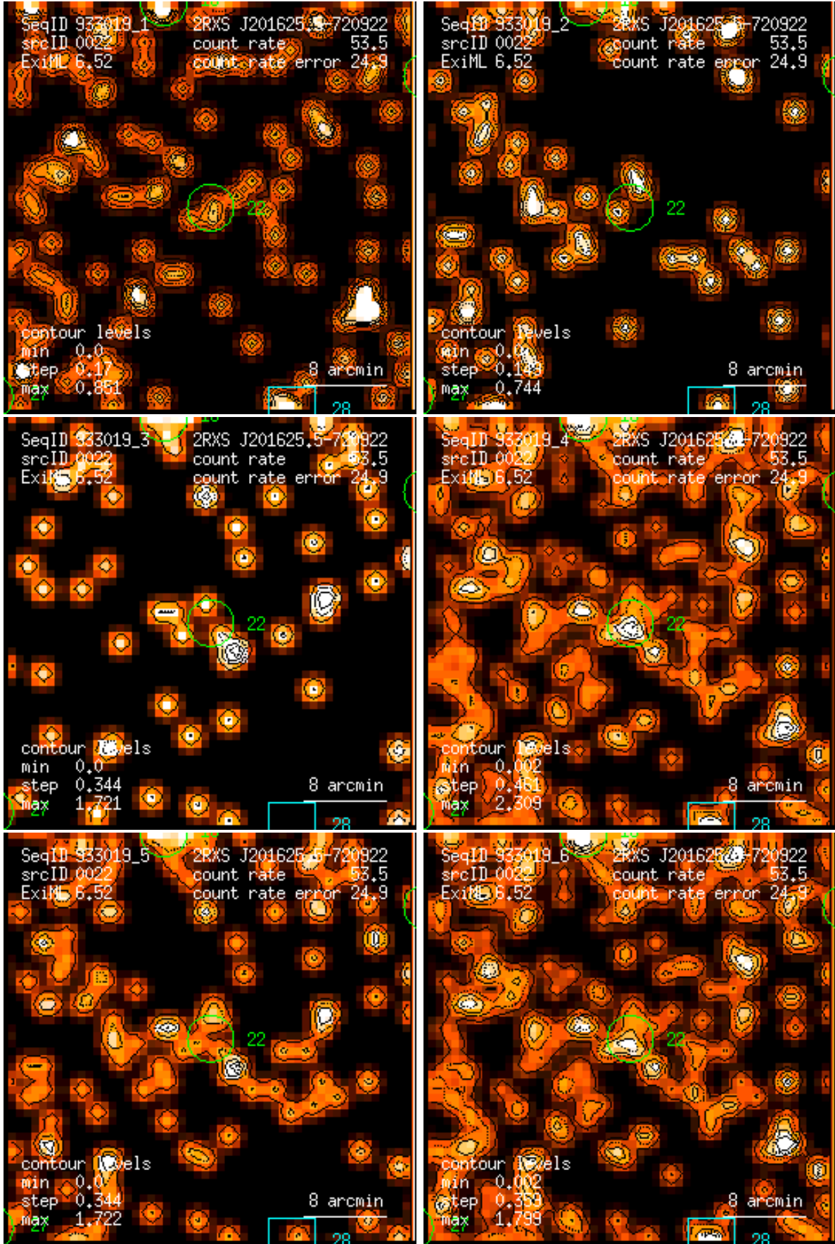
Figure 22: RASS 933019: detection 0022: band rate images, Gaussian filter: (1) PSPC channels 11 – 41, (2) 52 – 90, (3) 91 – 201, (4) 11 – 235, (5) 52 – 201, (6) 11 – 201. Broad band rates in counts/ks. Band rate contour levels in counts/ks/arcmin 2 .
