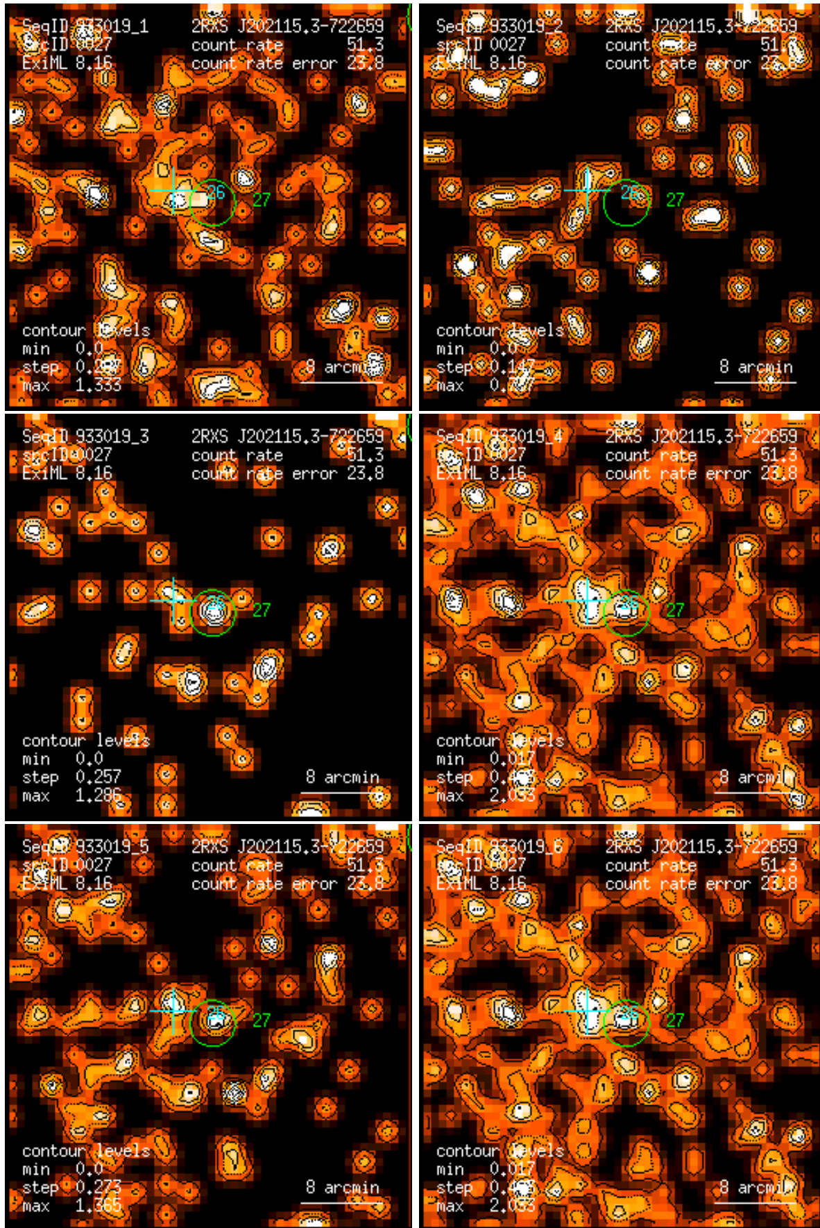
Figure 27: RASS 933019: detection 0027: band rate images, Gaussian filter: (1) PSPC channels 11 – 41, (2) 52 – 90, (3) 91 – 201, (4) 11 – 235, (5) 52 – 201, (6) 11 – 201. Broad band rates in counts/ks. Band rate contour levels in counts/ks/arcmin 2 .
