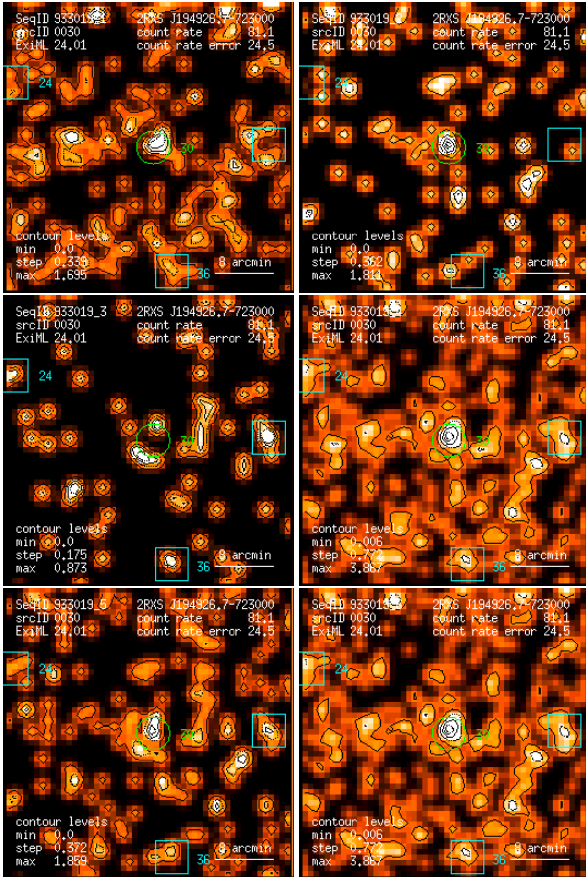
Figure 30: RASS 933019: detection 0030: band rate images, Gaussian filter: (1) PSPC channels 11 – 41, (2) 52 – 90, (3) 91 – 201, (4) 11 – 235, (5) 52 – 201, (6) 11 – 201. Broad band rates in counts/ks. Band rate contour levels in counts/ks/arcmin 2 .
