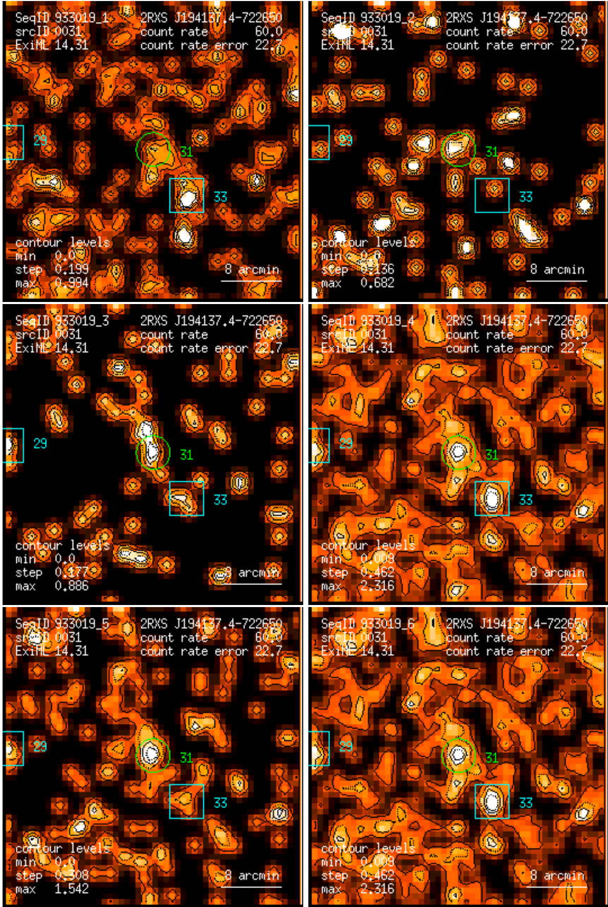
Figure 31: RASS 933019: detection 0031: band rate images, Gaussian filter: (1) PSPC channels 11 – 41, (2) 52 – 90, (3) 91 – 201, (4) 11 – 235, (5) 52 – 201, (6) 11 – 201. Broad band rates in counts/ks. Band rate contour levels in counts/ks/arcmin 2 .
