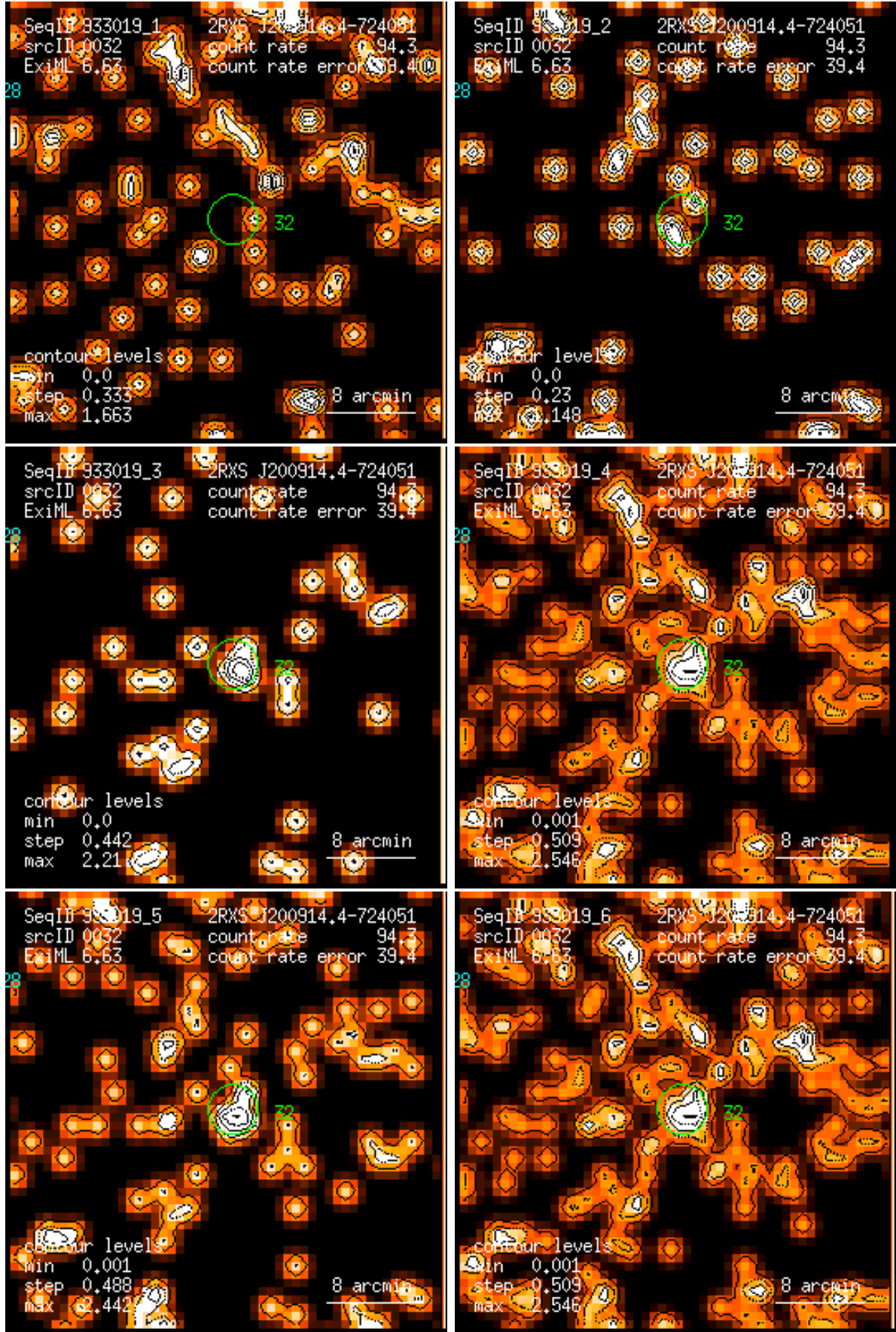
Figure 32: RASS 933019: detection 0032: band rate images, Gaussian filter: (1) PSPC channels 11 – 41, (2) 52 – 90, (3) 91 – 201, (4) 11 – 235, (5) 52 – 201, (6) 11 – 201. Broad band rates in counts/ks. Band rate contour levels in counts/ks/arcmin 2 .
