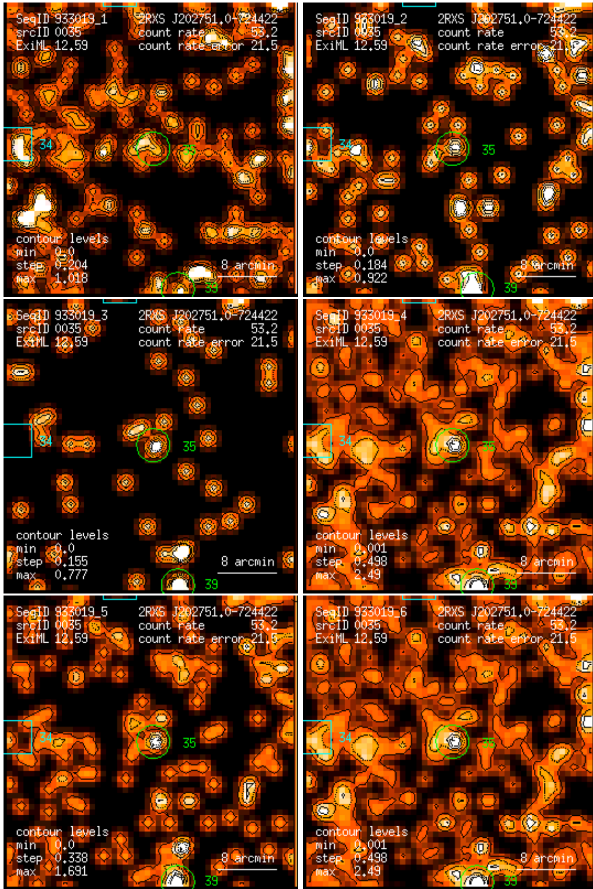
Figure 35: RASS 933019: detection 0035: band rate images, Gaussian filter: (1) PSPC channels 11 – 41, (2) 52 – 90, (3) 91 – 201, (4) 11 – 235, (5) 52 – 201, (6) 11 – 201. Broad band rates in counts/ks. Band rate contour levels in counts/ks/arcmin 2 .
