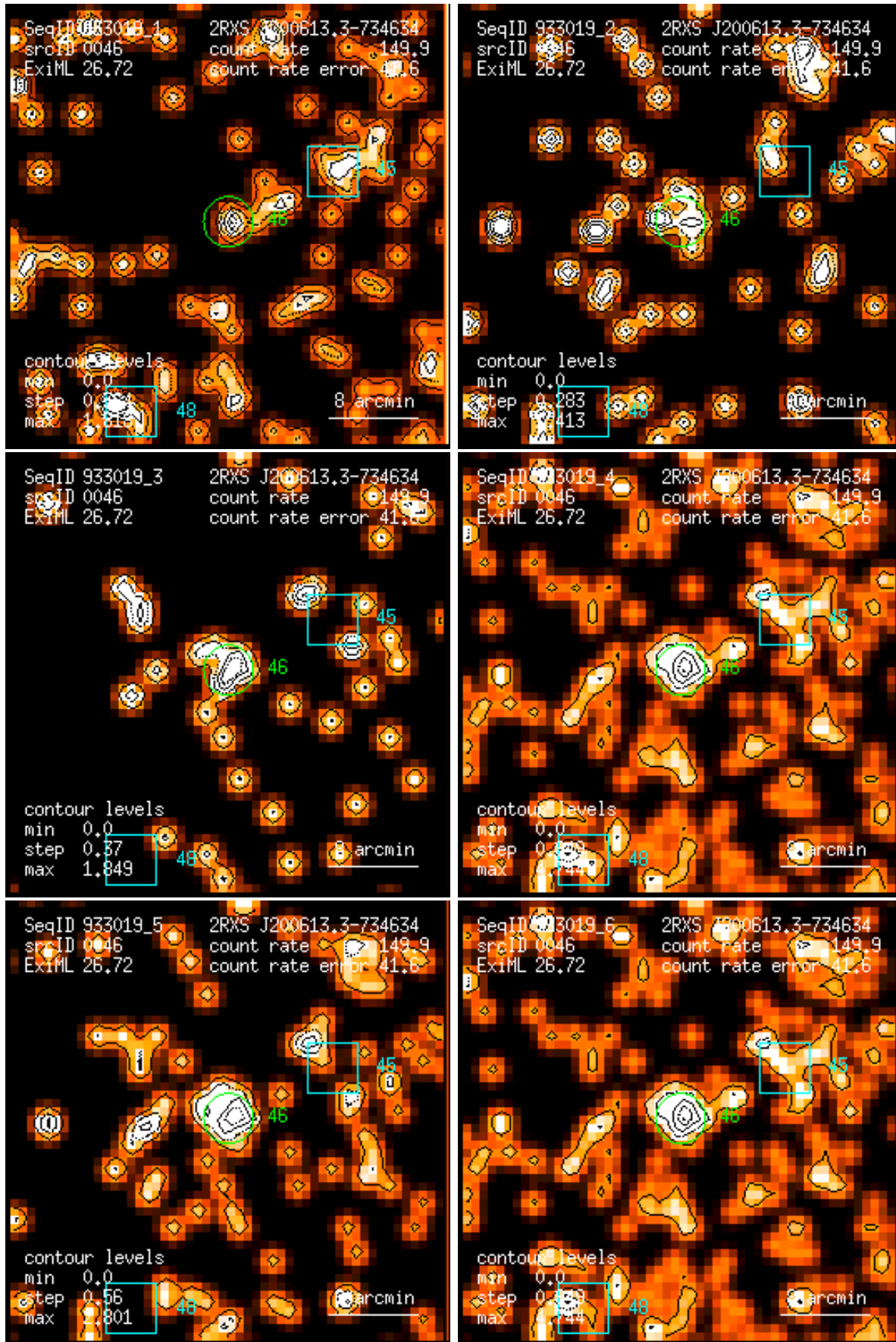
Figure 46: RASS 933019: detection 0046: band rate images, Gaussian filter: (1) PSPC channels 11 – 41, (2) 52 – 90, (3) 91 – 201, (4) 11 – 235, (5) 52 – 201, (6) 11 – 201. Broad band rates in counts/ks. Band rate contour levels in counts/ks/arcmin 2 .
