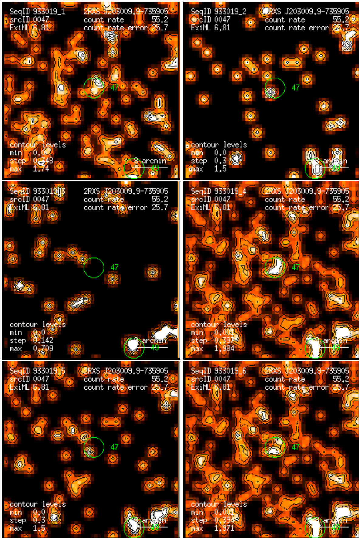
Figure 47: RASS 933019: detection 0047: band rate images, Gaussian filter: (1) PSPC channels 11 – 41, (2) 52 – 90, (3) 91 – 201, (4) 11 – 235, (5) 52 – 201, (6) 11 – 201. Broad band rates in counts/ks. Band rate contour levels in counts/ks/arcmin 2 .
