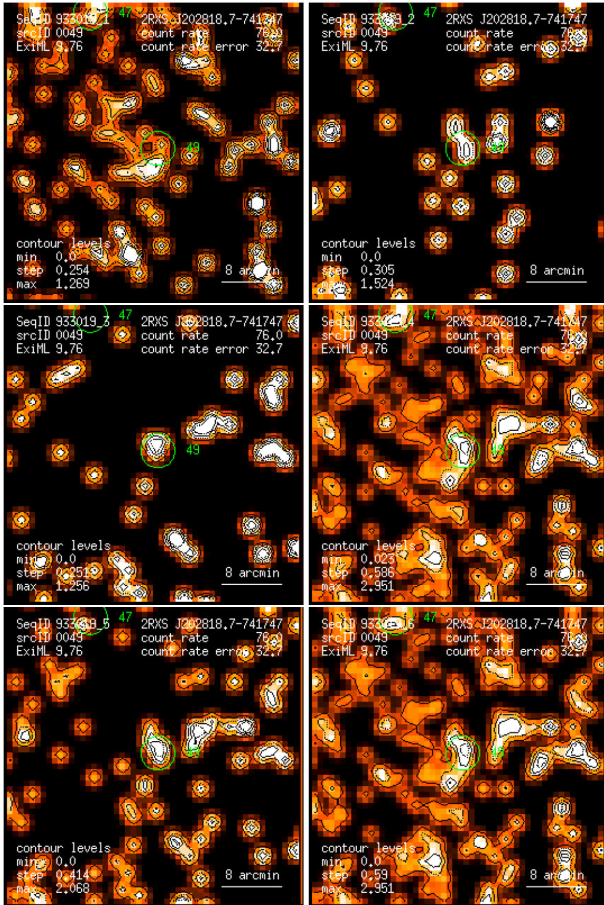
Figure 49: RASS 933019: detection 0049: band rate images, Gaussian filter: (1) PSPC channels 11 – 41, (2) 52 – 90, (3) 91 – 201, (4) 11 – 235, (5) 52 – 201, (6) 11 – 201. Broad band rates in counts/ks. Band rate contour levels in counts/ks/arcmin 2 .
