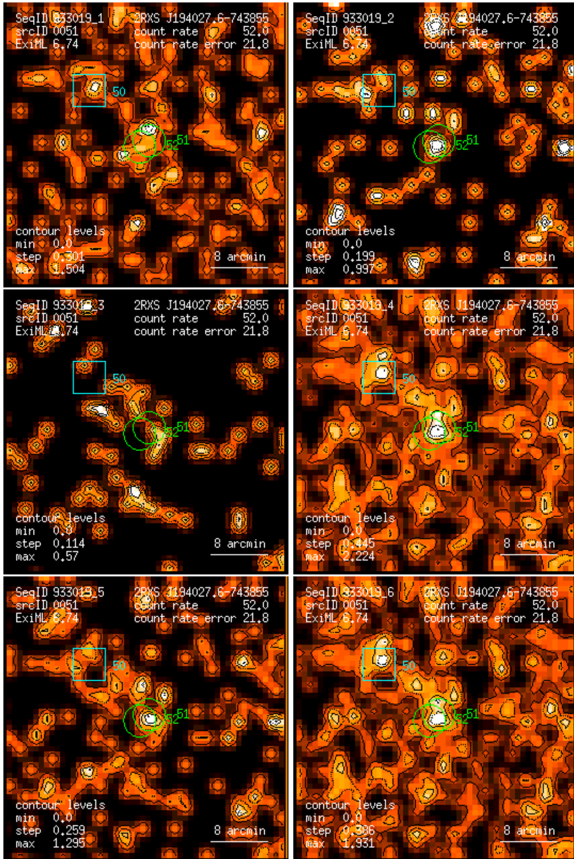
Figure 51: RASS 933019: detection 0051: band rate images, Gaussian filter: (1) PSPC channels 11 – 41, (2) 52 – 90, (3) 91 – 201, (4) 11 – 235, (5) 52 – 201, (6) 11 – 201. Broad band rates in counts/ks. Band rate contour levels in counts/ks/arcmin 2 .
