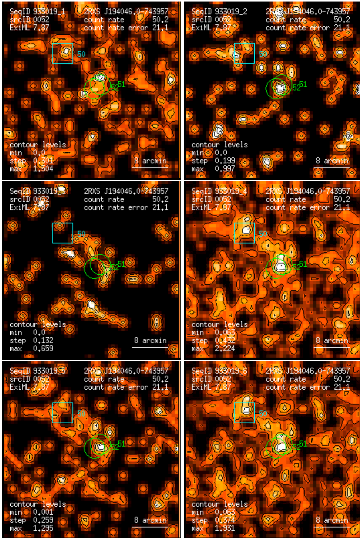
Figure 52: RASS 933019: detection 0052: band rate images, Gaussian filter: (1) PSPC channels 11 – 41, (2) 52 – 90, (3) 91 – 201, (4) 11 – 235, (5) 52 – 201, (6) 11 – 201. Broad band rates in counts/ks. Band rate contour levels in counts/ks/arcmin 2 .
