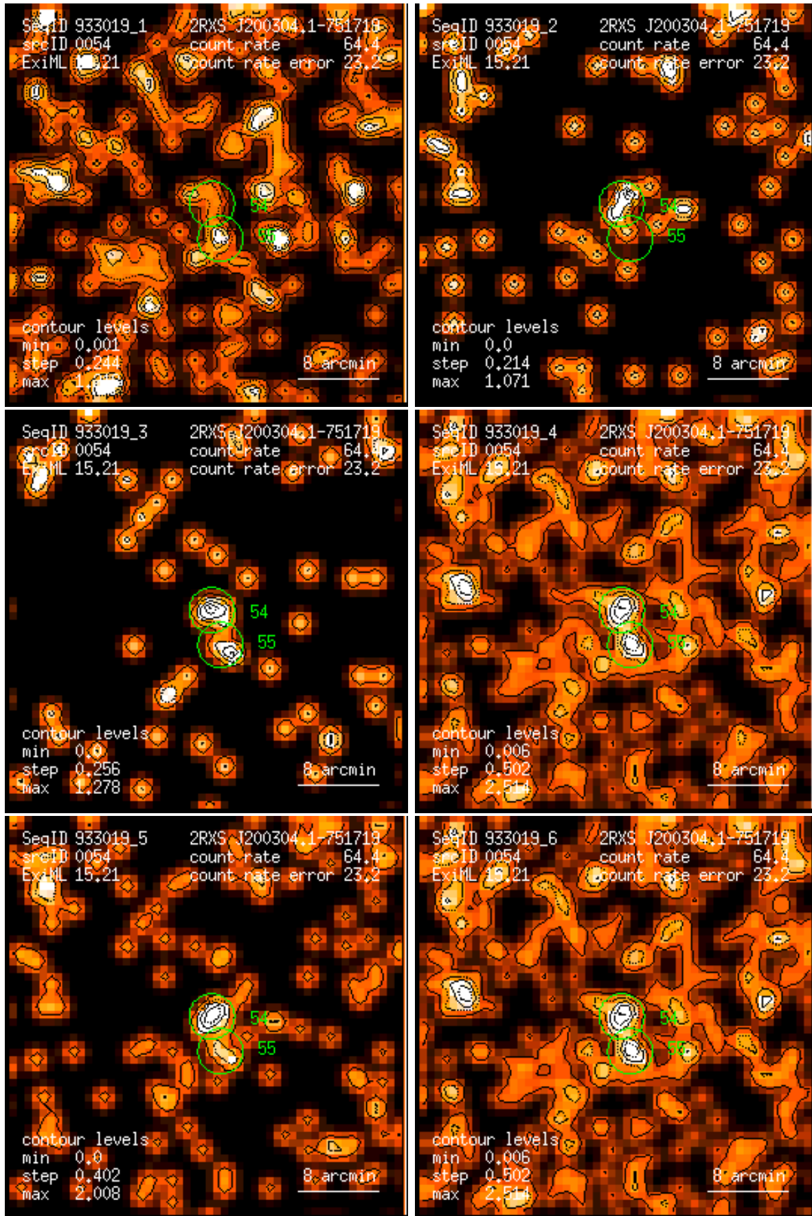
Figure 54: RASS 933019: detection 0054: band rate images, Gaussian filter: (1) PSPC channels 11 – 41, (2) 52 – 90, (3) 91 – 201, (4) 11 – 235, (5) 52 – 201, (6) 11 – 201. Broad band rates in counts/ks. Band rate contour levels in counts/ks/arcmin 2 .
