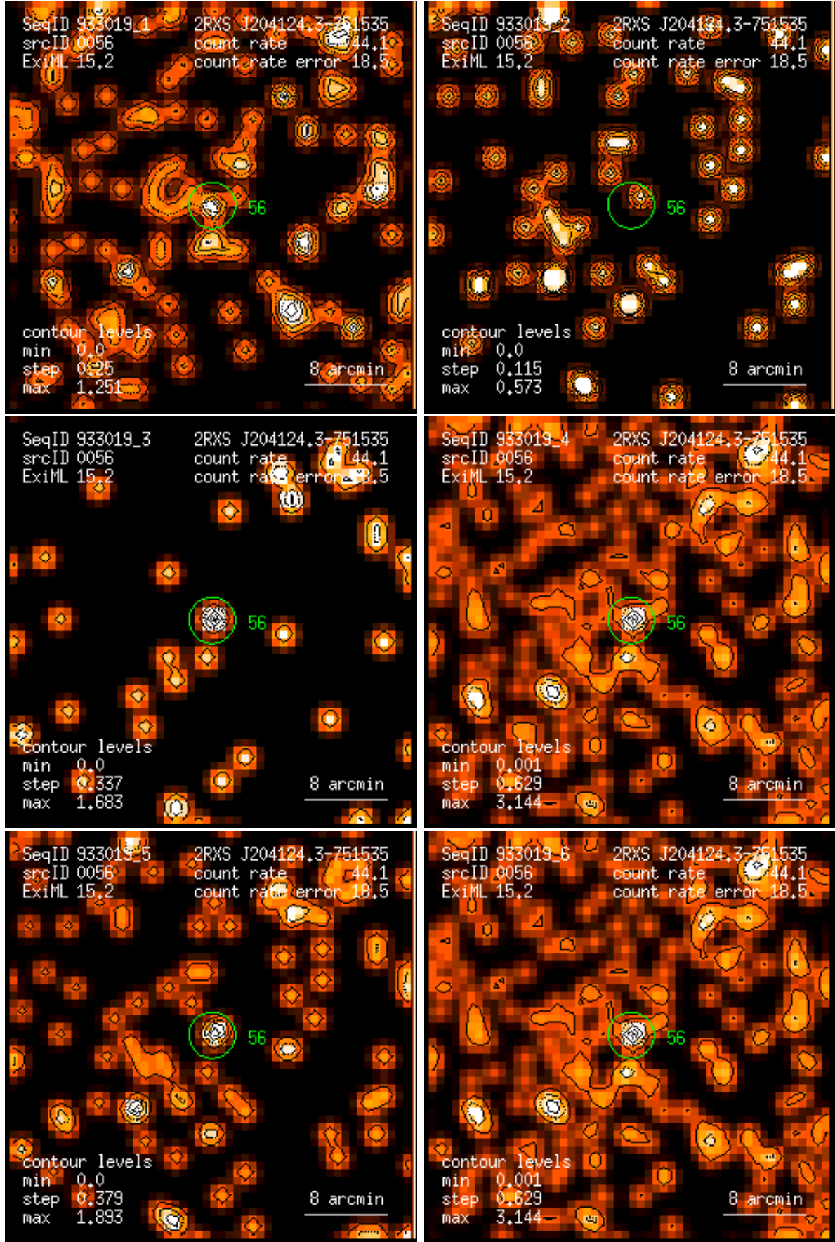
Figure 56: RASS 933019: detection 0056: band rate images, Gaussian filter: (1) PSPC channels 11 – 41, (2) 52 – 90, (3) 91 – 201, (4) 11 – 235, (5) 52 – 201, (6) 11 – 201. Broad band rates in counts/ks. Band rate contour levels in counts/ks/arcmin 2 .
