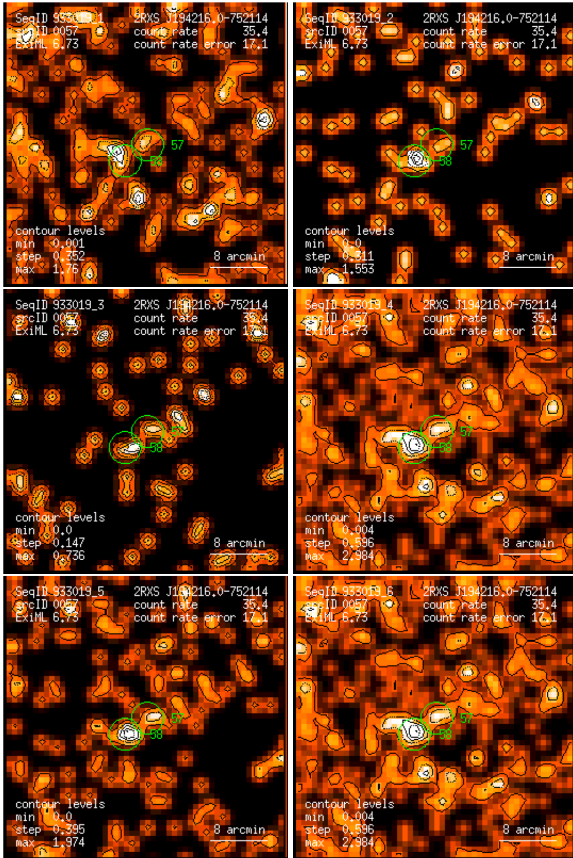
Figure 57: RASS 933019: detection 0057: band rate images, Gaussian filter: (1) PSPC channels 11 – 41, (2) 52 – 90, (3) 91 – 201, (4) 11 – 235, (5) 52 – 201, (6) 11 – 201. Broad band rates in counts/ks. Band rate contour levels in counts/ks/arcmin 2 .
