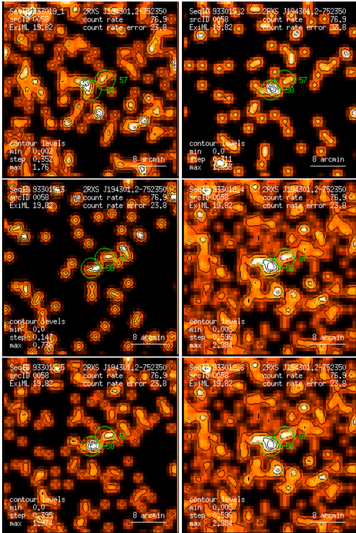
Figure 58: RASS 933019: detection 0058: band rate images, Gaussian filter: (1) PSPC channels 11 – 41, (2) 52 – 90, (3) 91 – 201, (4) 11 – 235, (5) 52 – 201, (6) 11 – 201. Broad band rates in counts/ks. Band rate contour levels in counts/ks/arcmin 2 .
