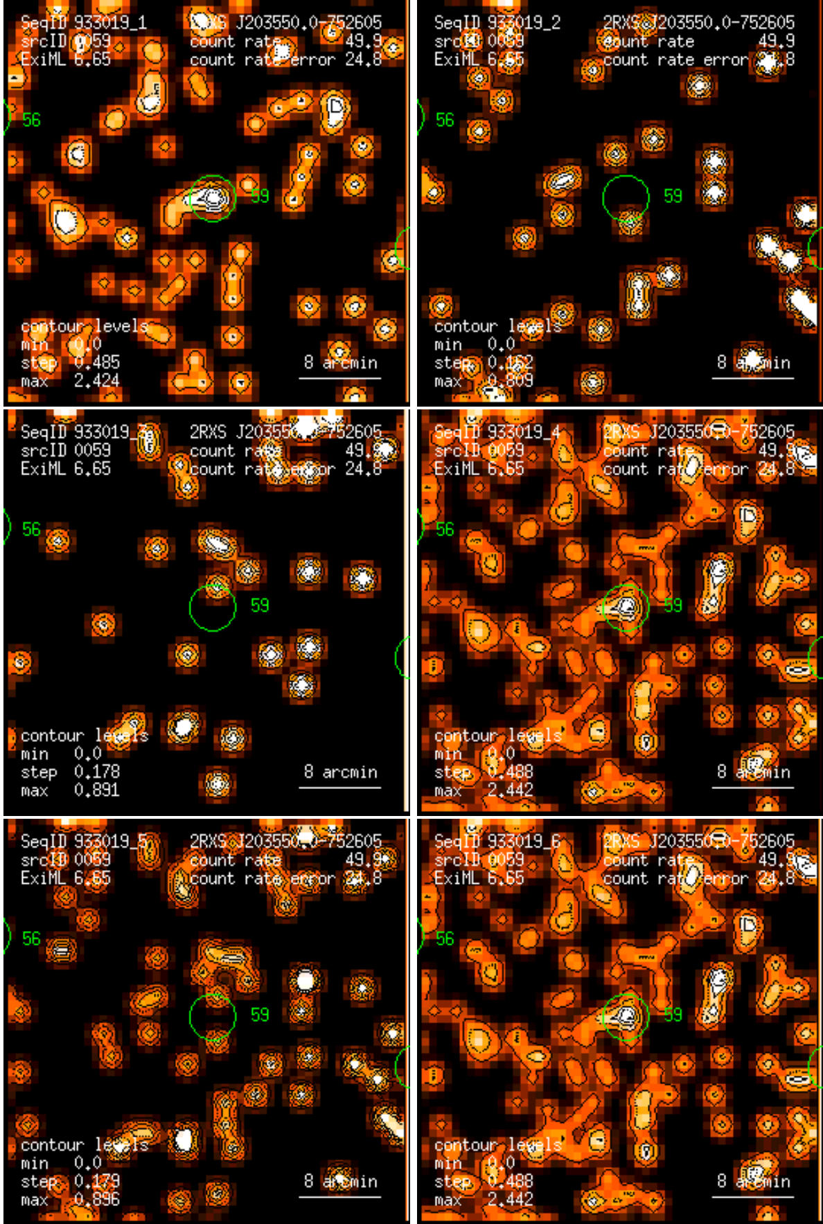
Figure 59: RASS 933019: detection 0059: band rate images, Gaussian filter: (1) PSPC channels 11 – 41, (2) 52 – 90, (3) 91 – 201, (4) 11 – 235, (5) 52 – 201, (6) 11 – 201. Broad band rates in counts/ks. Band rate contour levels in counts/ks/arcmin 2 .
