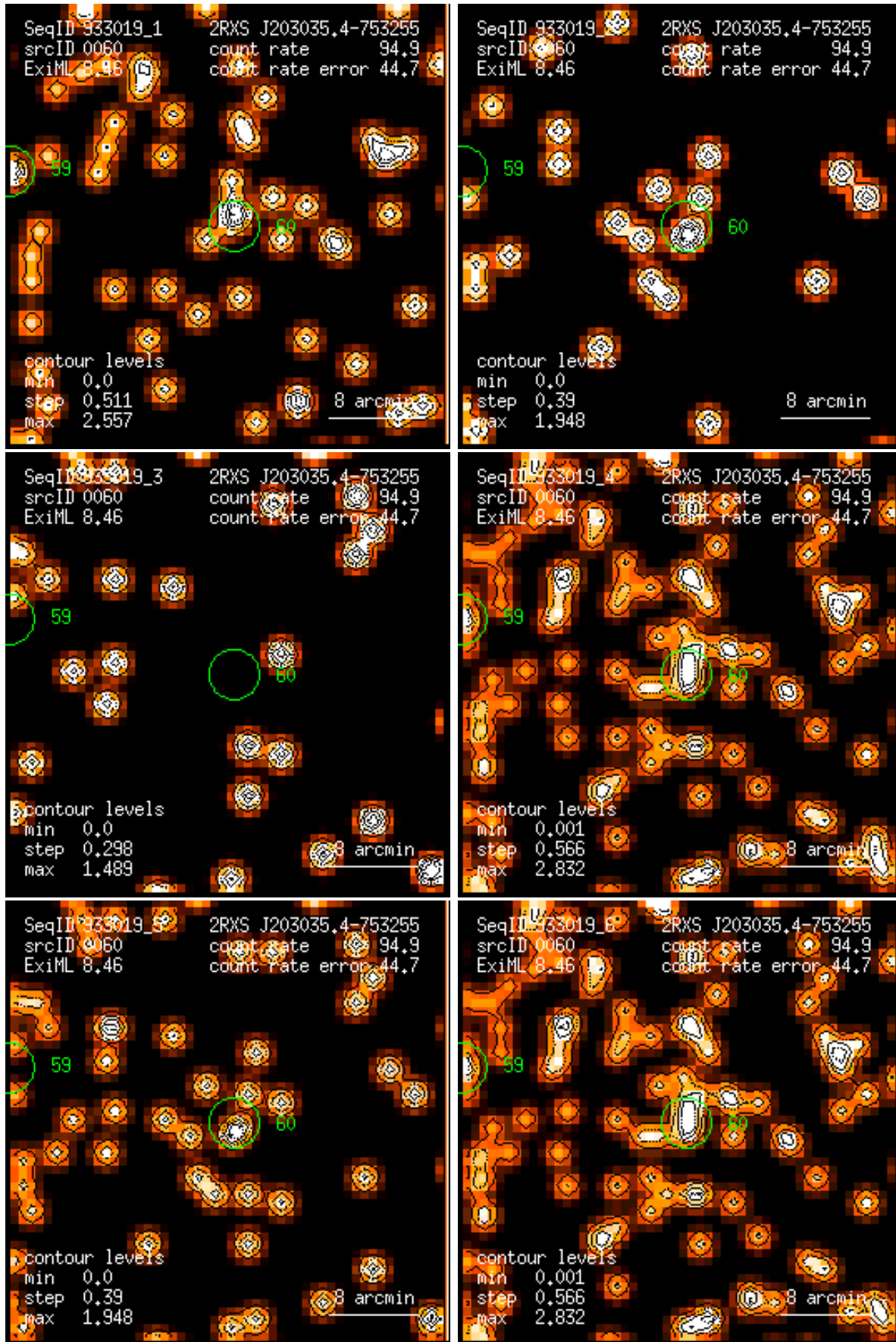
Figure 60: RASS 933019: detection 0060: band rate images, Gaussian filter: (1) PSPC channels 11 – 41, (2) 52 – 90, (3) 91 – 201, (4) 11 – 235, (5) 52 – 201, (6) 11 – 201. Broad band rates in counts/ks. Band rate contour levels in counts/ks/arcmin 2 .
