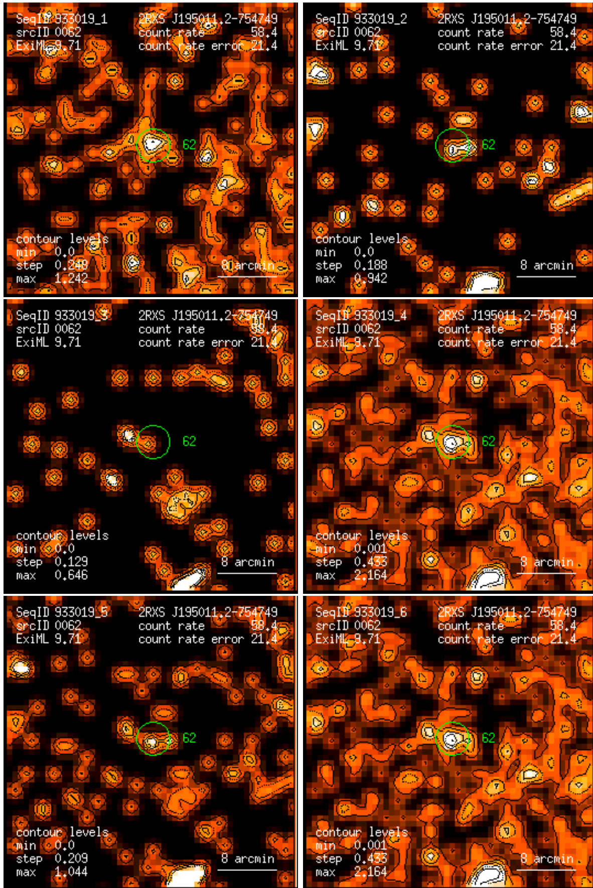
Figure 62: RASS 933019: detection 0062: band rate images, Gaussian filter: (1) PSPC channels 11 – 41, (2) 52 – 90, (3) 91 – 201, (4) 11 – 235, (5) 52 – 201, (6) 11 – 201. Broad band rates in counts/ks. Band rate contour levels in counts/ks/arcmin 2 .
