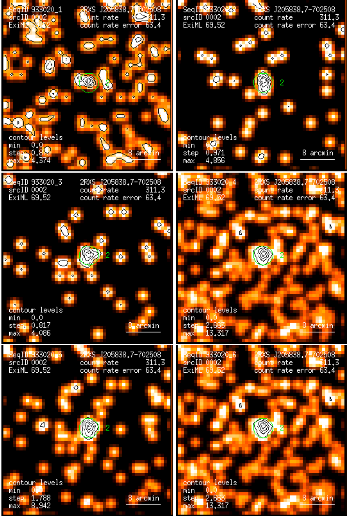
Figure 2: RASS 933020: detection 0002: band rate images, Gaussian filter: (1) PSPC channels 11 – 41, (2) 52 – 90, (3) 91 – 201, (4) 11 – 235, (5) 52 – 201, (6) 11 – 201. Broad band rates in counts/ks. Band rate contour levels in counts/ks/arcmin 2 .
